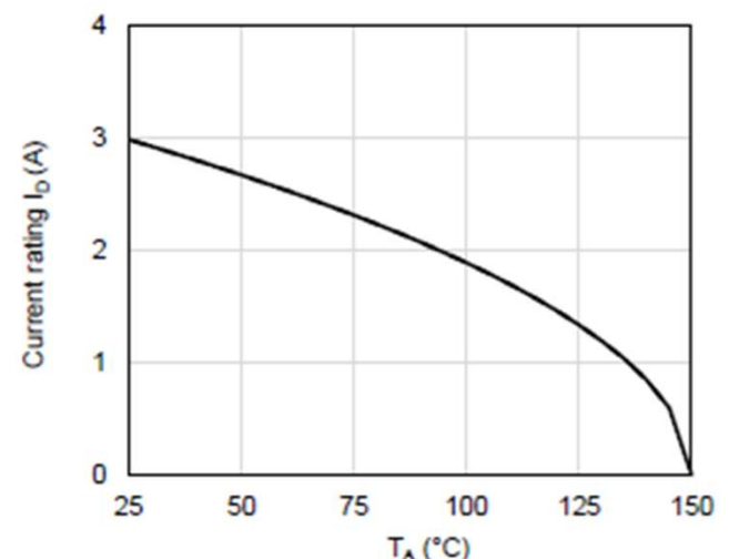
Figure 12: Current De-rating
