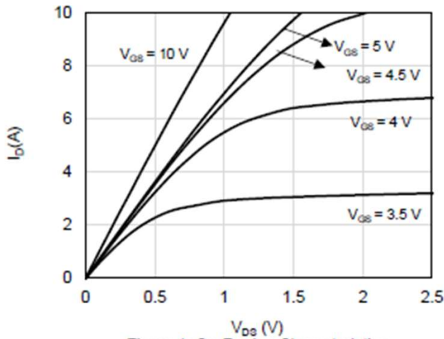
Figure 1: On-Region Characteristics
