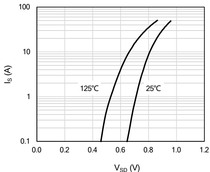
Figure 7: Body-Diode Characteristics
