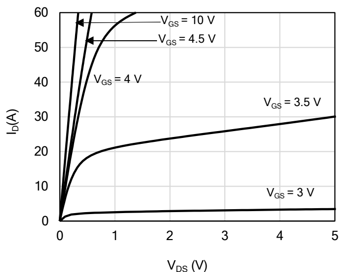
Figure 1: On-Region Characteristics
