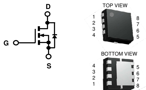
DFN3.3x3.3
