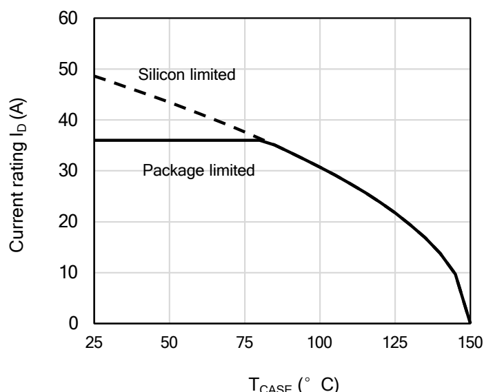
Figure 12: Current De-rating
