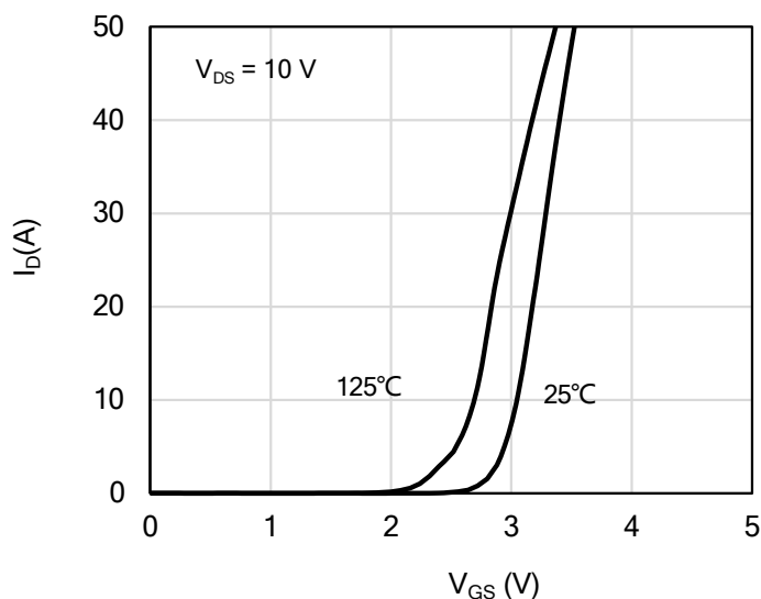
Figure 2: Transfer Characteristics
