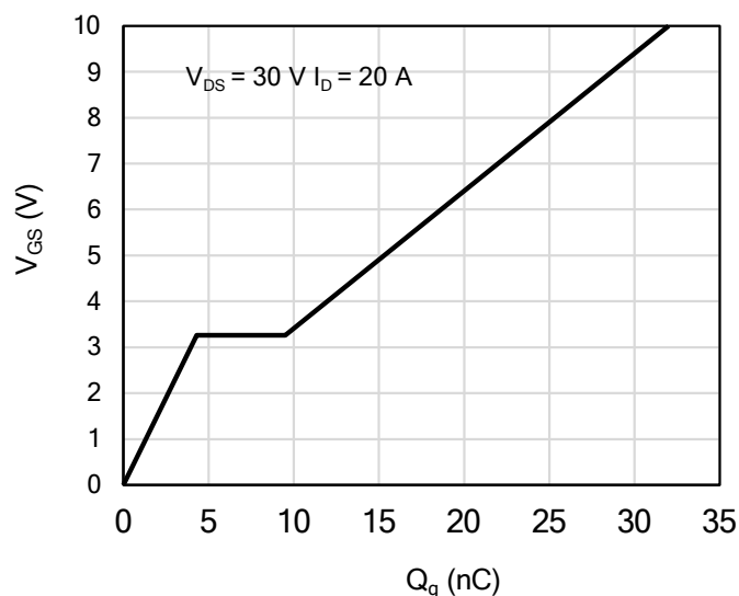
Figure 10: Gate-Charge Characteristics
