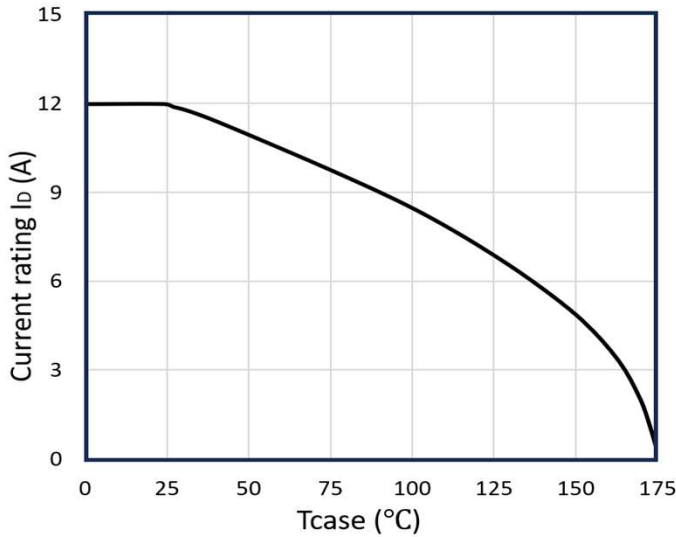
Figure 19: Current De-rating
