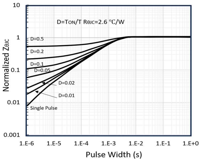
Figure 21: Normalized Maximum Transient Thermal Impedance
