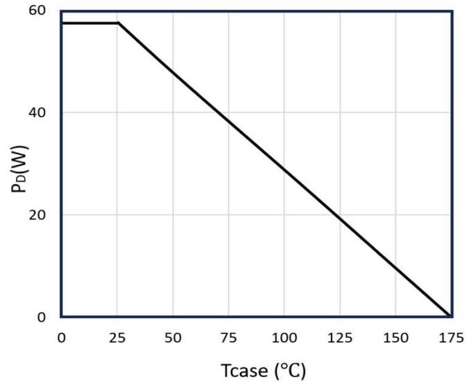
Figure 20: Maximum Power Dissipation Derating vs. Case Temperature
