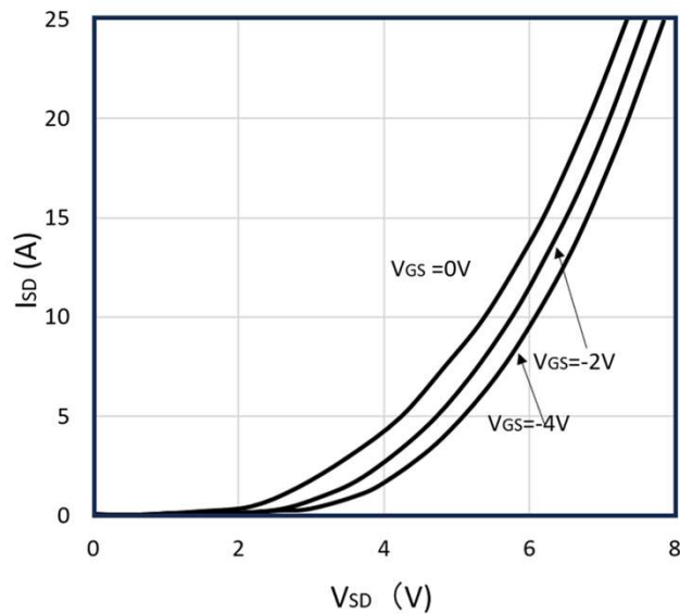
Figure 9: Body Diode Characteristics at 25^\circ C
