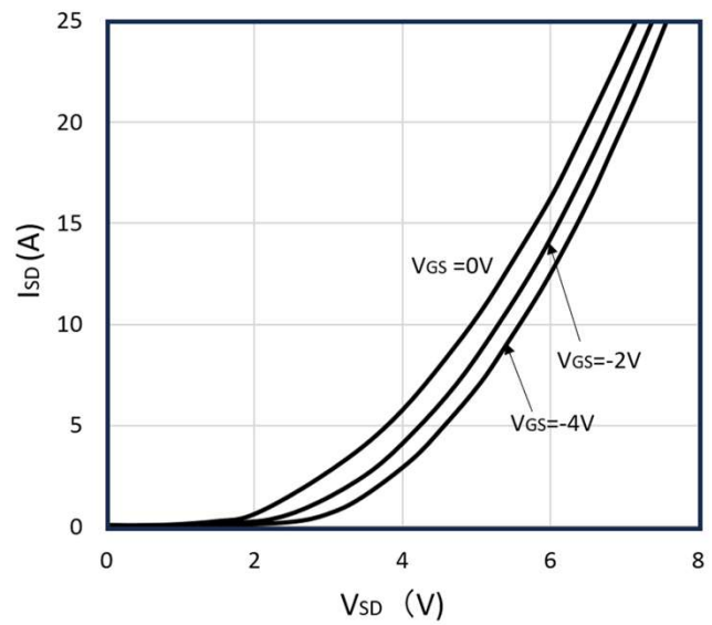
Figure 10: Body Diode Characteristics at 175^\circ C
