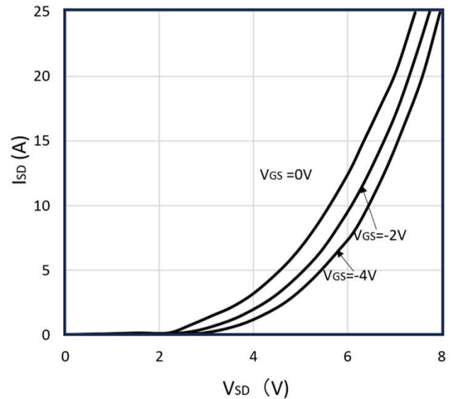
Figure 8: Body Diode Characteristics at -40^\circ C
