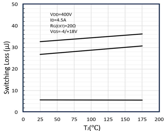
Figure 24: Clamped Inductive Switching Energy vs T J
