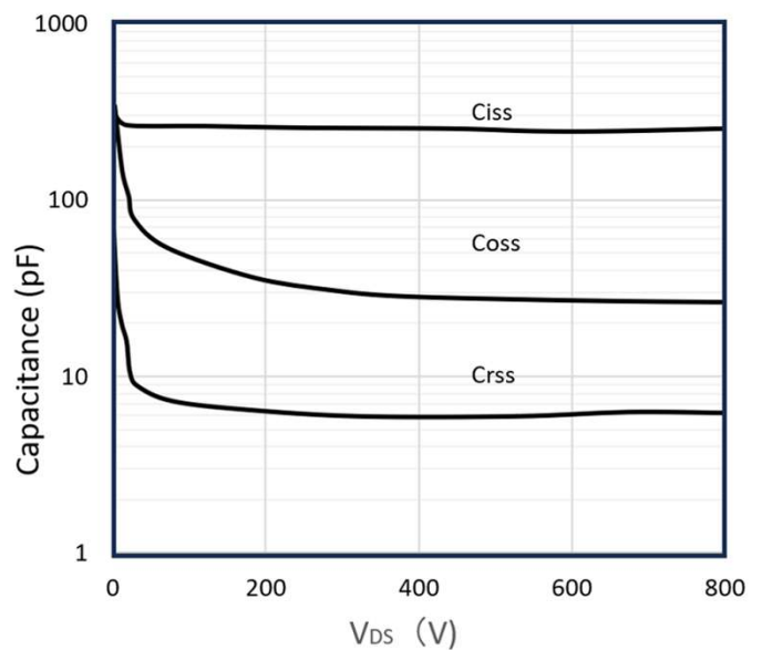
Figure 18: Capacitance Characteristics(0 - 800V)
