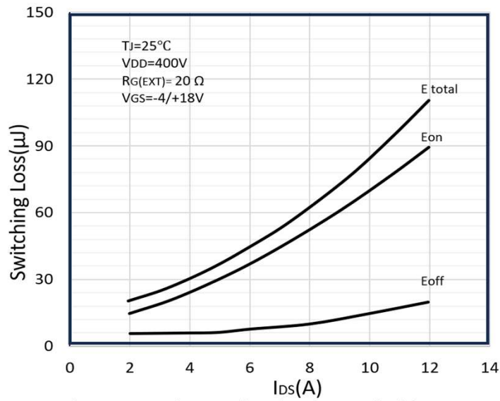
Figure 25: Clamped Inductive Switching Energy vs. Drain Current (VDD=400V)
