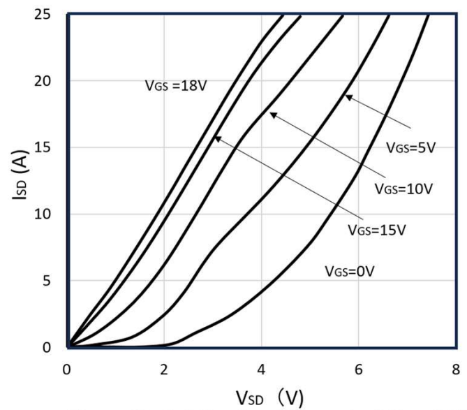
Figure 14: 3rd Quadrant Characteristics at 25°C
