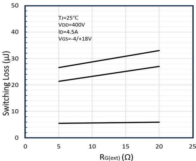
Figure 23: Clamped Inductive Switching Energy vs R G(EXT)
