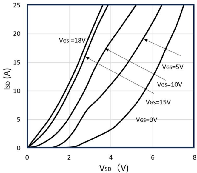
Figure 13: 3rd Quadrant Characteristics at -40°C
