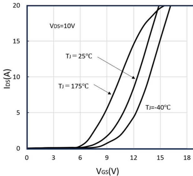
Figure 7: Transfer Characteristics For Various Junction Temperature
