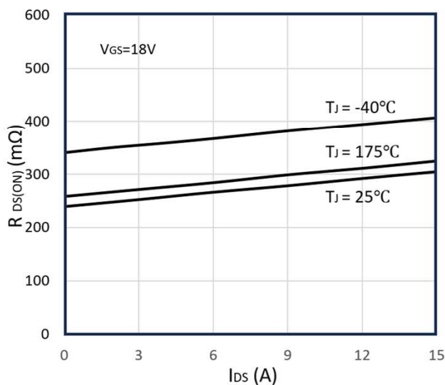
Figure 5: On-Resistance vs. Drain Current For Various Temperatures
