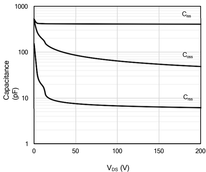
Figure 17: Capacitance Characteristics (0 - 200 V)
