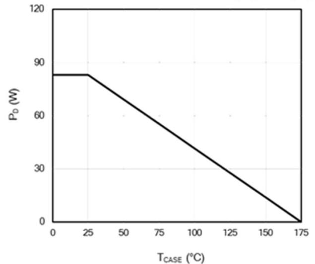
Figure 20: Maximum Power Dissipation Derating vs. Case Temperature
