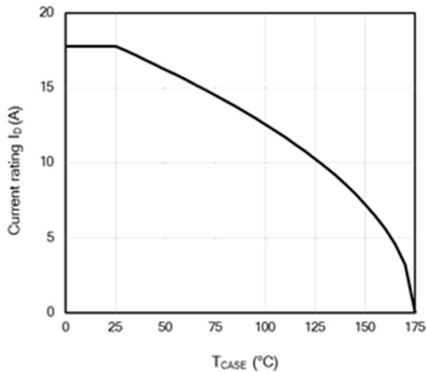
Figure 19: Current De-rating
