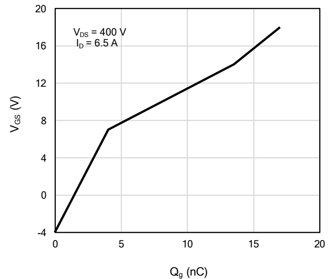
Figure 12: Gate-Charge Characteristics
