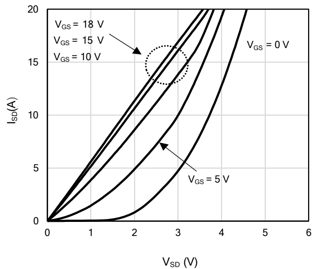
Figure 15: 3rd Quadrant Characteristics at 175^{\circ}\text{C}
