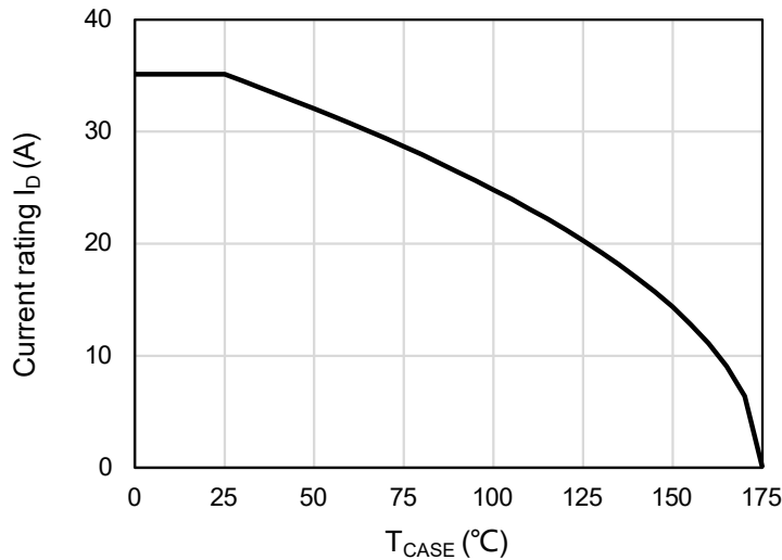
Figure 19: Current De-rating
