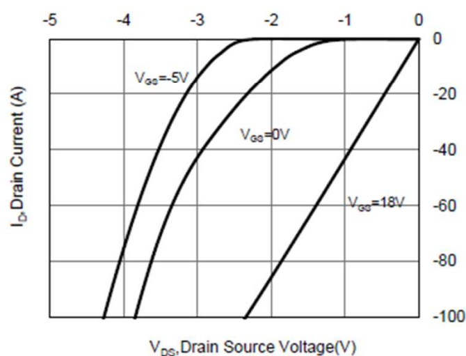
Fig 12. 3rd Quadrant Characteristic at 175 °C
