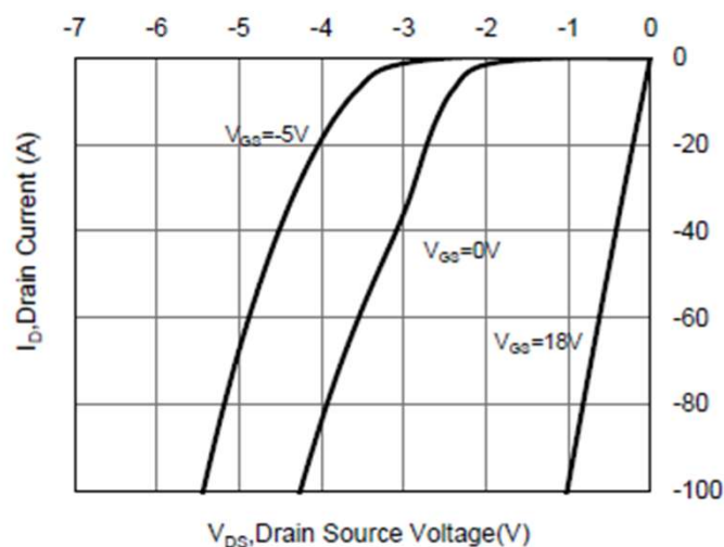
Fig 10. 3rd Quadrant Characteristic at -55 °C
