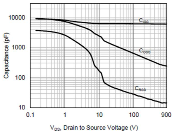
Fig 8. Capacitance Characteristics
