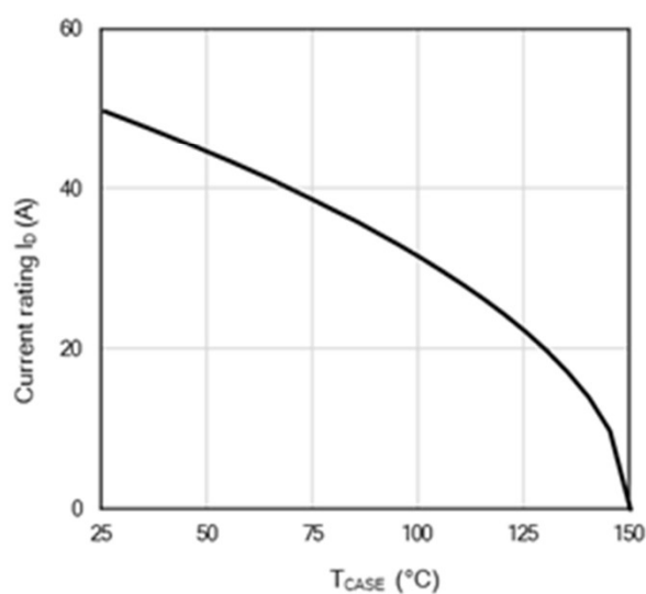
Figure 12: Current De-rating
