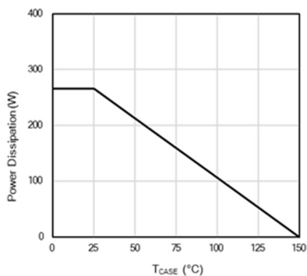
Figure 11: Power De-rating
