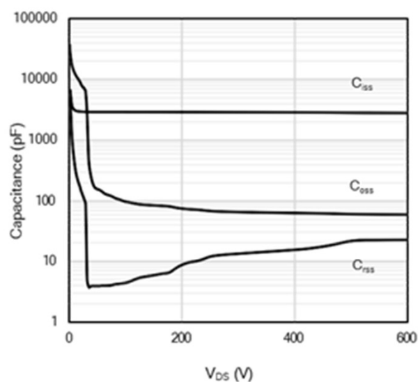
Figure 9: Capacitance Characteristics
