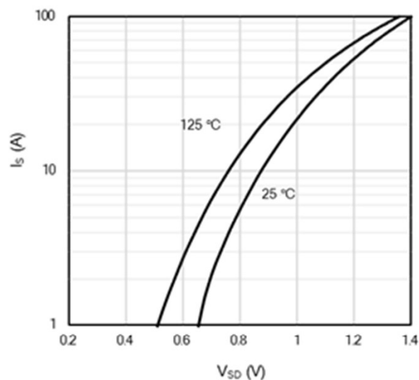
Figure 7: Body-Diode Characteristics
