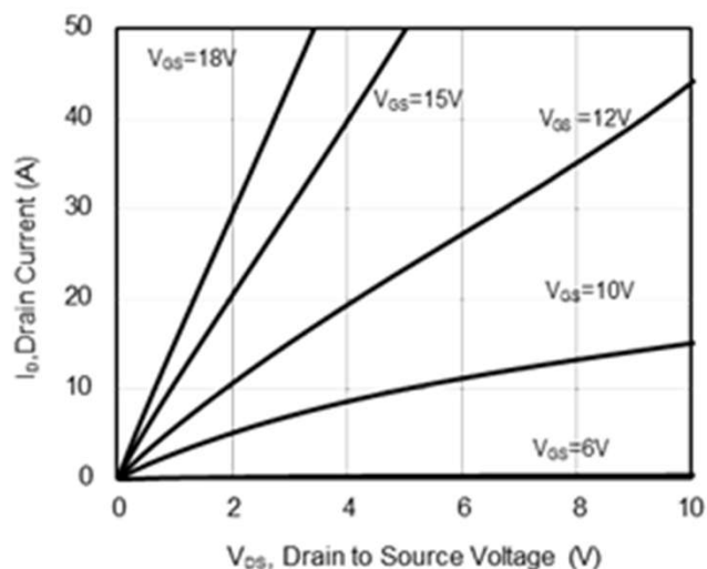
Fig 1. Output Characteristics, T_j = -55^\circ\text{C}
