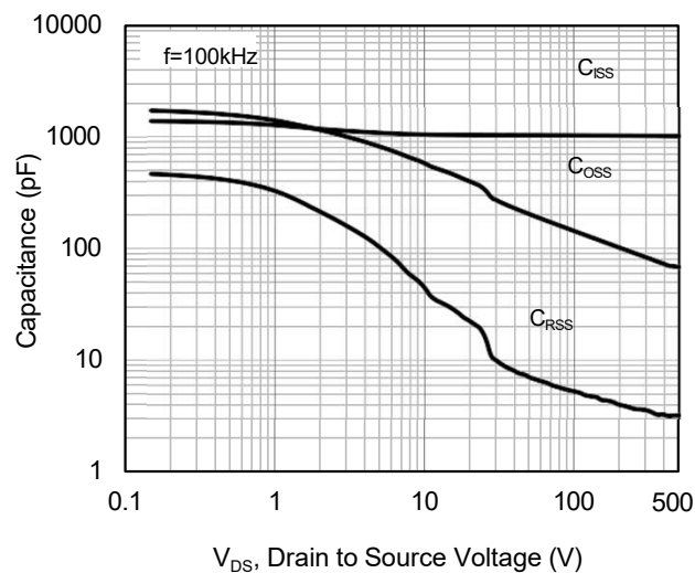
Fig 8. Capacitance Characteristics
