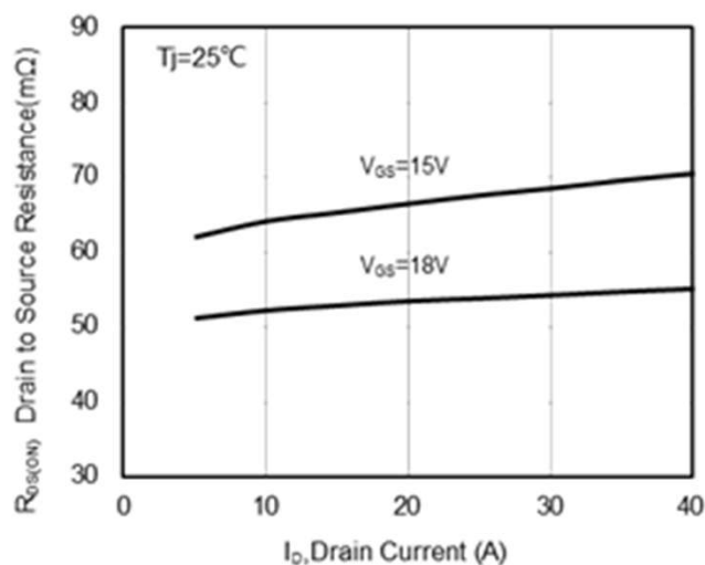
Fig 6. On-Resistance vs Drain Current
