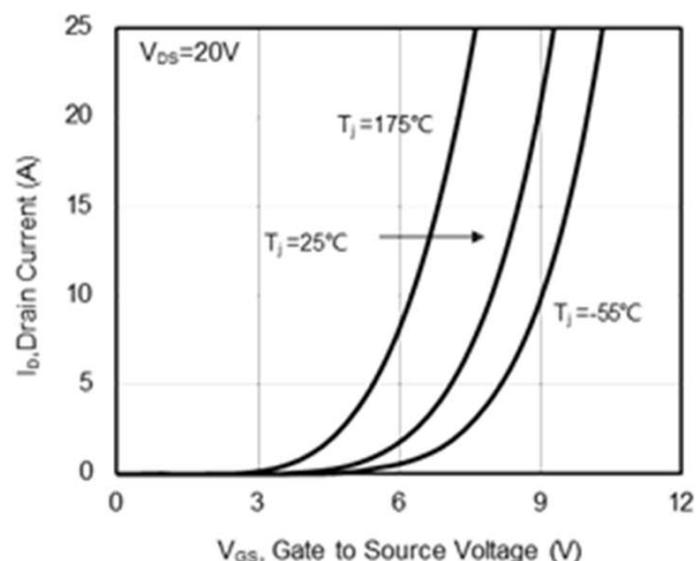
Fig 4. Transfer Characteristics
