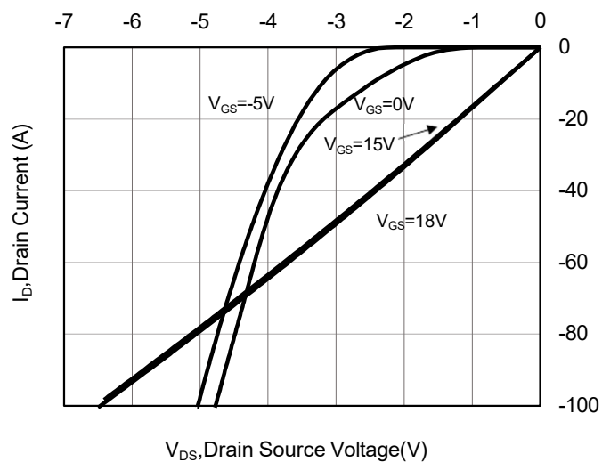
Fig 14. 3rd Quadrant Characteristic at 175 °C
