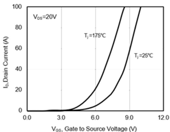
Fig 3. Transfer Characteristics
