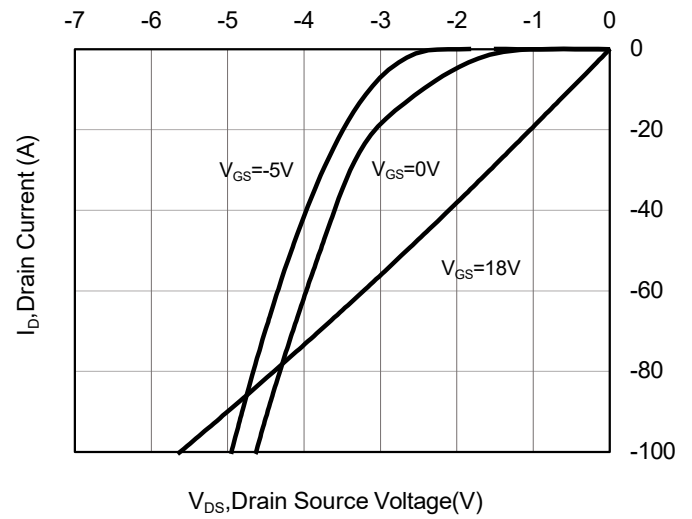
Fig 10. 3rd Quadrant Characteristic at 175 °C
