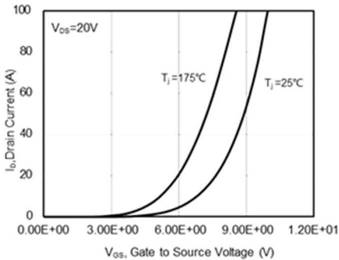
Fig 3. Transfer Characteristics
