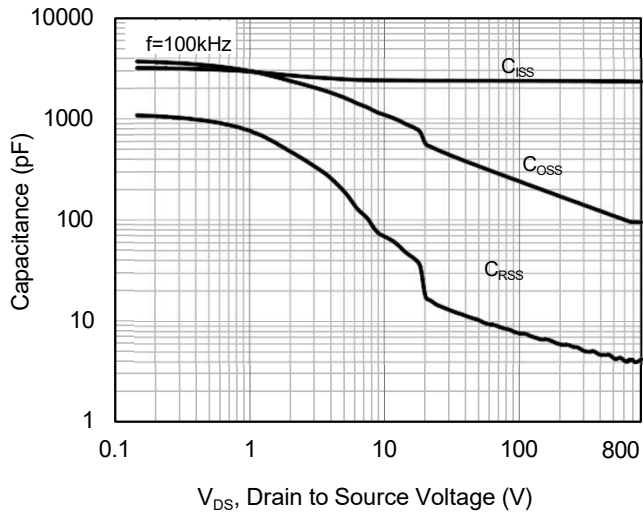
Fig 7. Capacitance Characteristics
