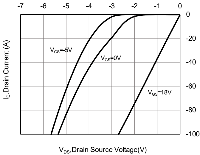
Fig 9. 3rd Quadrant Characteristic at 25 °C
