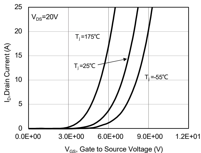
Fig 4. Transfer Characteristics
