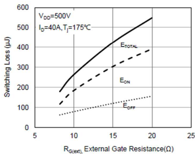
Fig 12. Switching Energy vs. Gate Resistance
