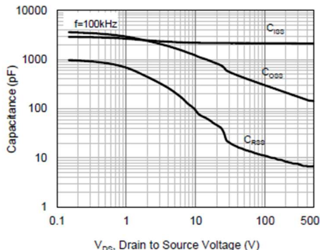
Fig 8. Capacitance Characteristics
