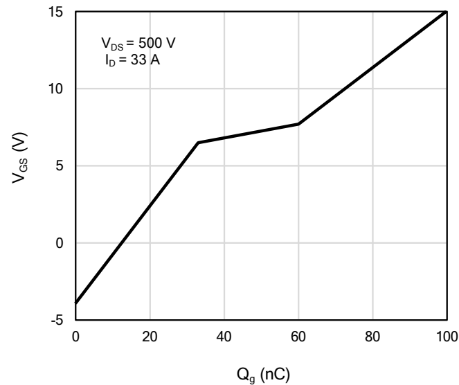
Figure 12: Gate-Charge Characteristics
