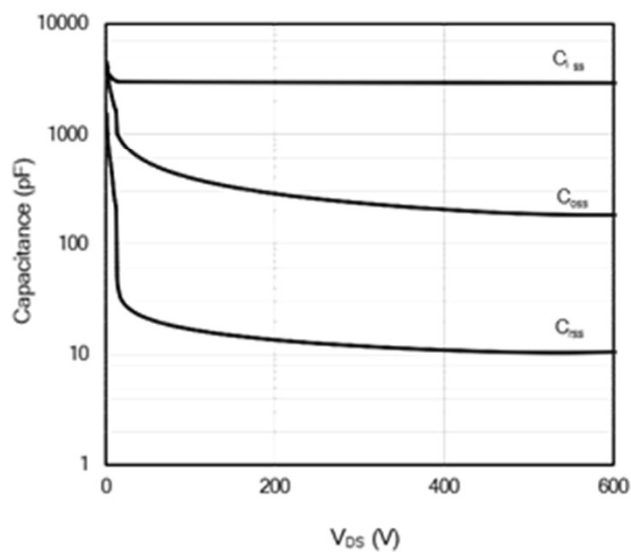
Figure 18: Capacitance Characteristics (0 - 600 V)
