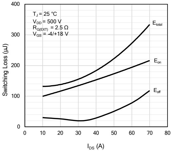
Figure 25: Clamped Inductive Switching Energy vs. Drain Current ( V_{DD} = 500\text{ V} )
