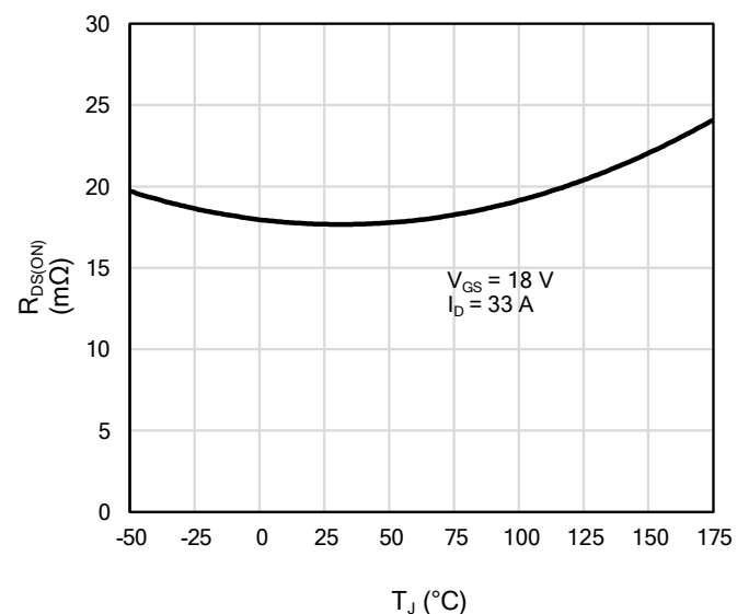
Figure 6: On-Resistance vs. Temperature
