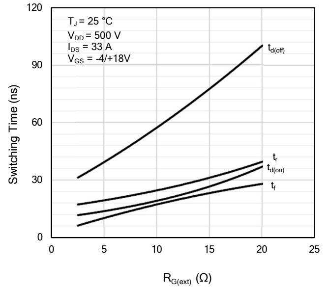
Figure 26: Switching Times vs. R_{G(EXT)}
