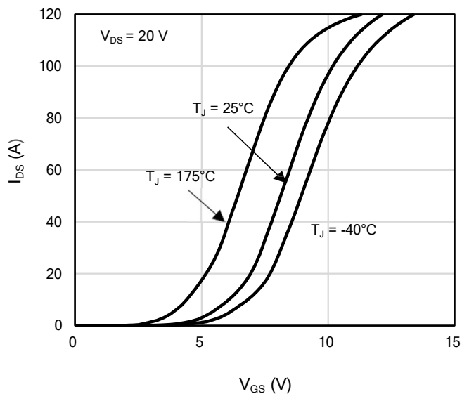
Figure 7: Transfer Characteristics For Various Junction Temperatures
