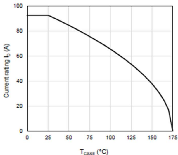
Figure 19: Current De-rating
