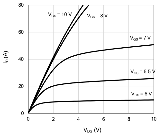
Figure 1: On-Region Characteristics
