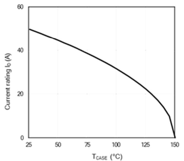
Figure 12: Current De-rating
