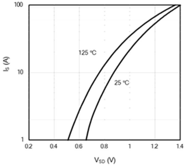
Figure 7: Body-Diode Characteristics
