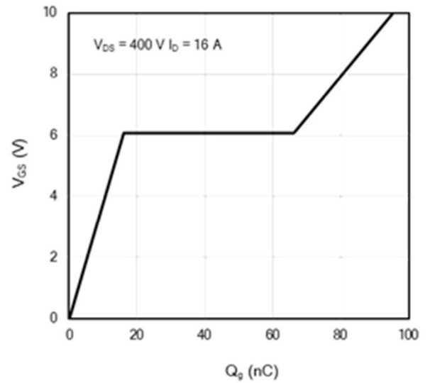
Figure 10: Gate-Charge Characteristics
