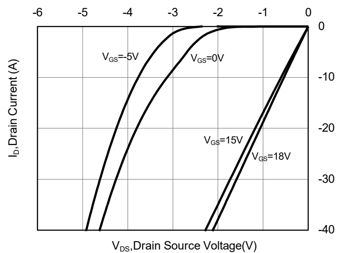
Fig 14. 3rd Quadrant Characteristic at 25 °C
