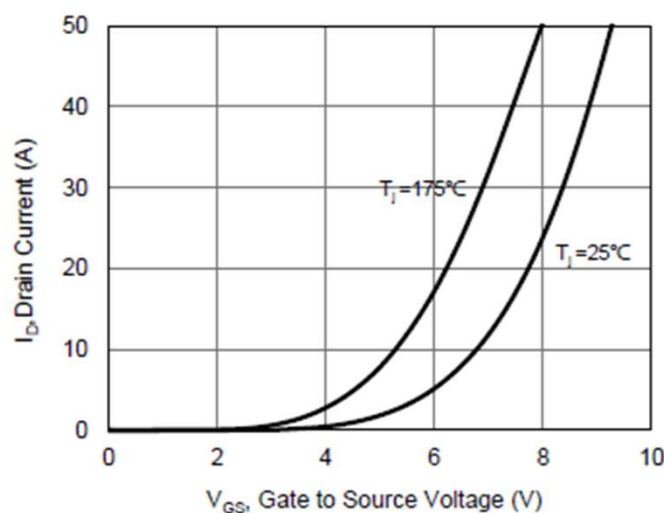
Fig 4: Transfer Characteristics
