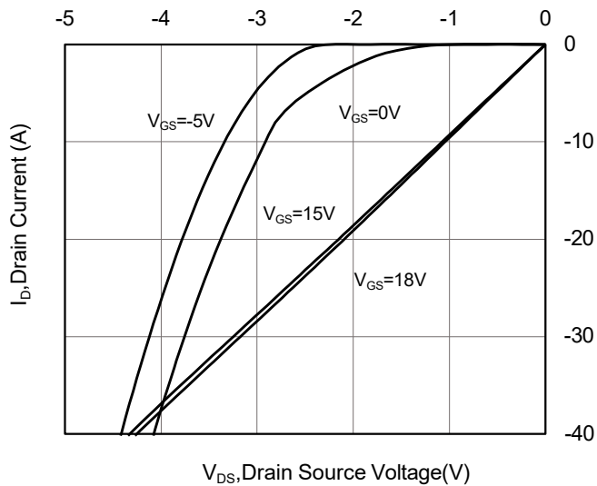
Fig 15. 3rd Quadrant Characteristic at 175 °C
