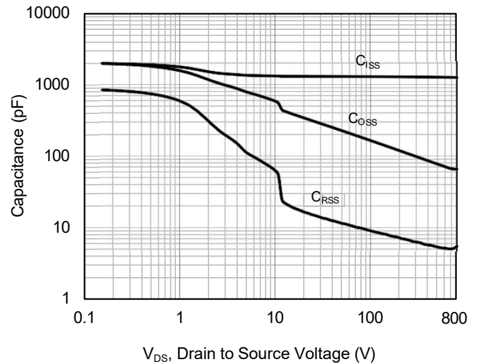
Fig 8. Capacitance Characteristics
