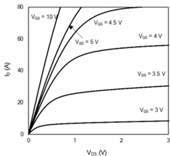
Figure 1: On-Region Characteristics
