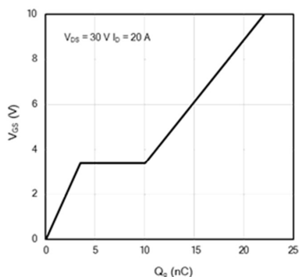
Figure 10: Gate-Charge Characteristics
