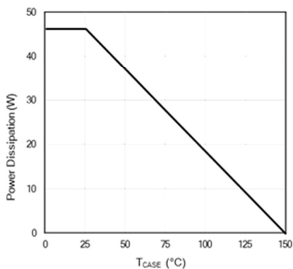
Figure 11: Power De-rating
