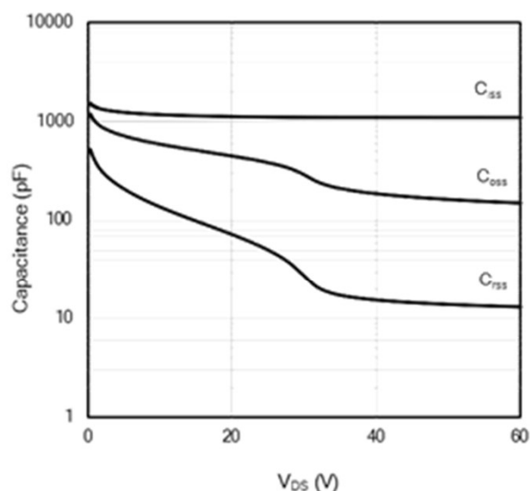
Figure 9: Capacitance Characteristics
