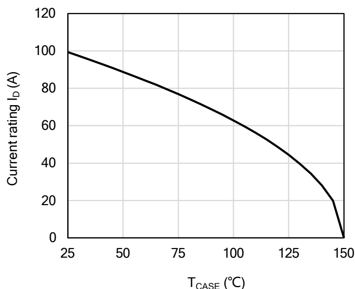
Figure 12: Current De-rating
