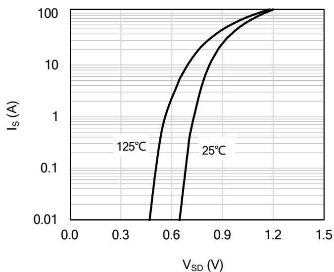
Figure 7: Body-Diode Characteristics
