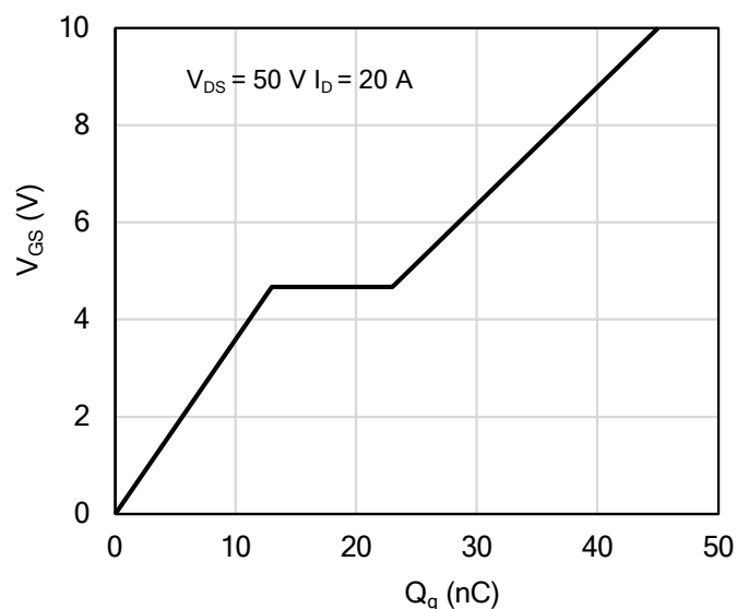
Figure 10: Gate-Charge Characteristics
