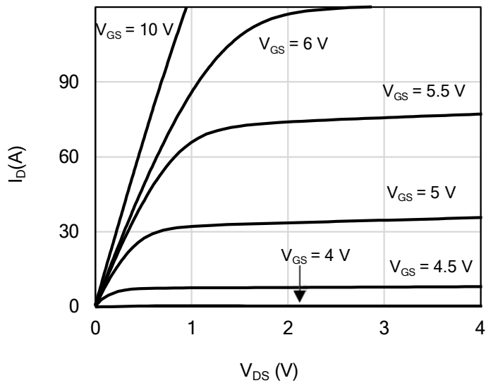
Figure 1: On-Region Characteristics
