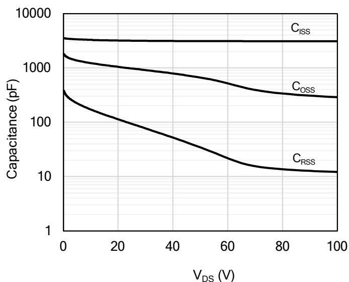
Figure 9: Capacitance Characteristics
