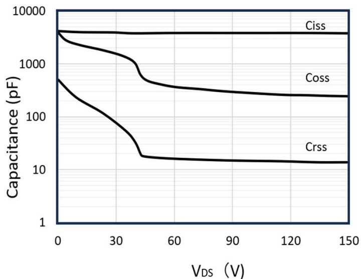
Figure 9: Capacitance Characteristics
