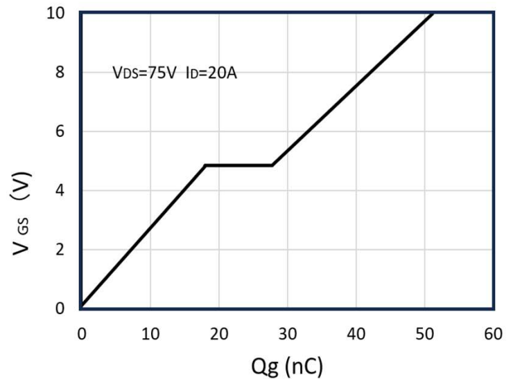
Figure 10: Gate-Charge Characteristics
