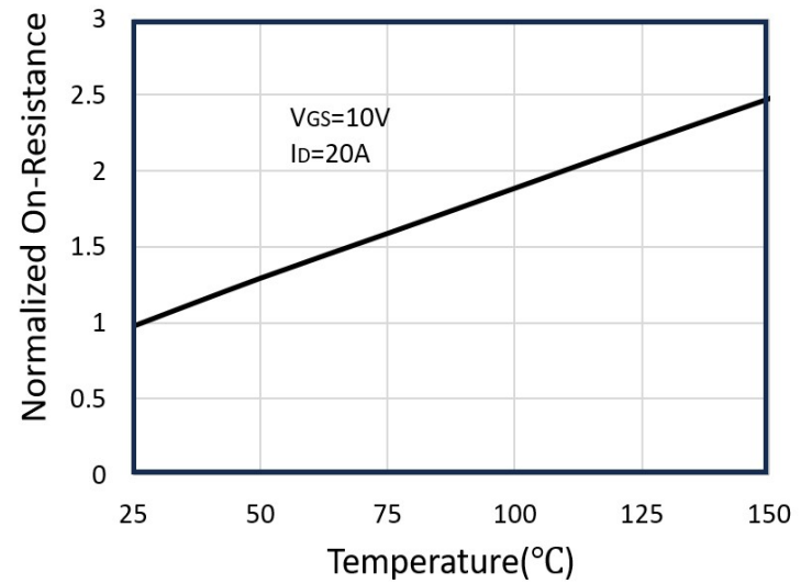
Figure 4: On-Resistance vs. Junction Temperature
