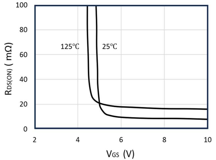
Figure 8: On-Resistance vs. Gate-Source Voltage
