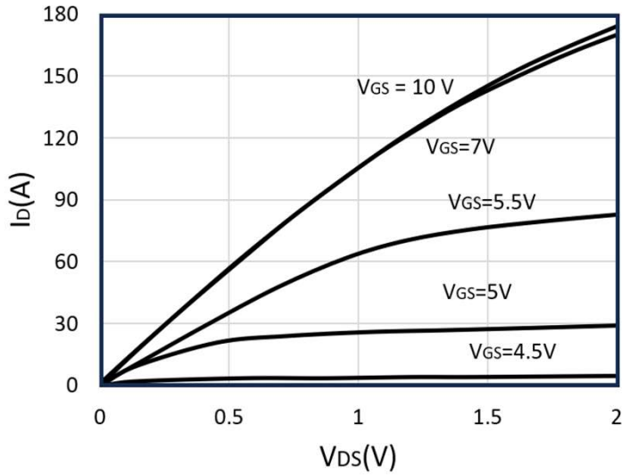
Figure 1: On-Region Characteristics
