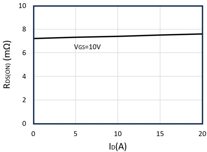
Figure 3: On- Resistance vs. Drain Current and Gate Voltage
