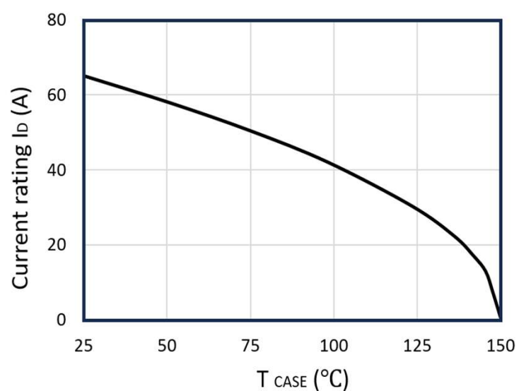
Figure 12: Current De-rating
