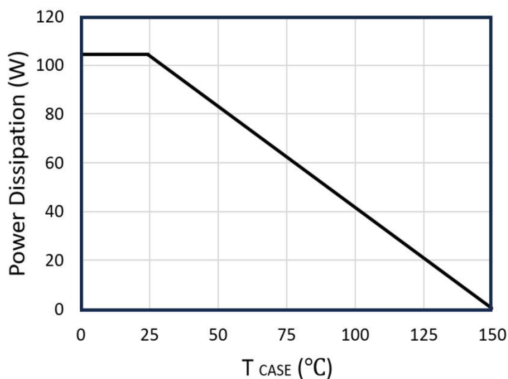
Figure 11: Power De-rating
