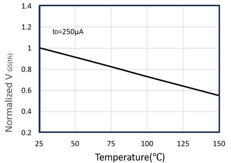
Figure 6: Threshold Voltage vs. Junction Temperature
