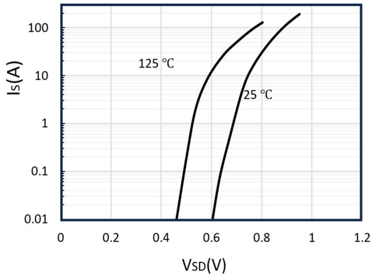
Figure 7: Body-Diode Characteristics
