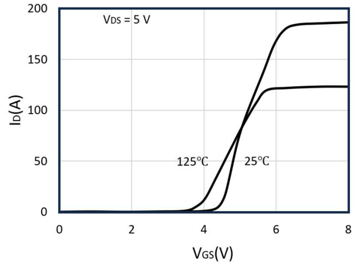
Figure 2: Transfer Characteristic
