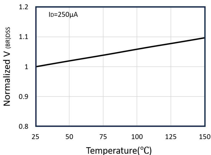
Figure 5: Breakdown Voltage vs. Junction Temperature
