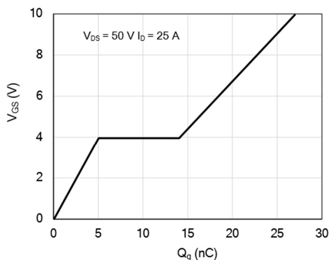
Figure 10: Gate-Charge Characteristics
