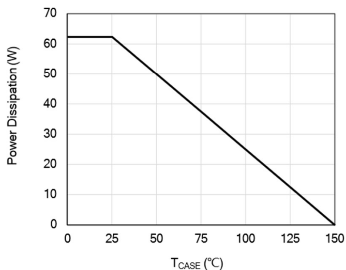
Figure 11: Power De-rating
