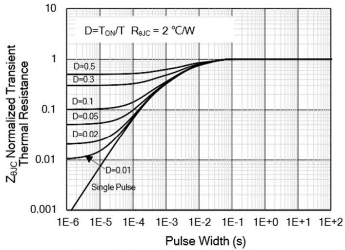
Figure 13: Normalized Maximum Transient Thermal Impedance
