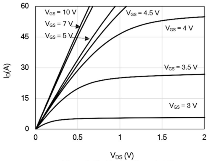
Figure 1: On-Region Characteristics
