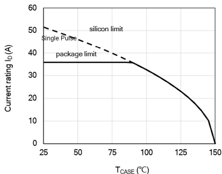
Figure 12: Current De-rating
