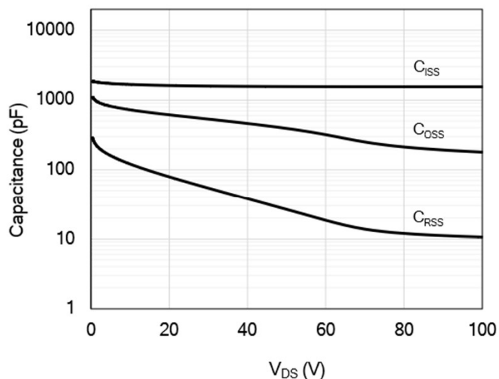
Figure 9: Capacitance Characteristics
