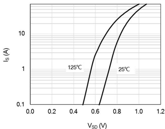
Figure 7: Body-Diode Characteristics
