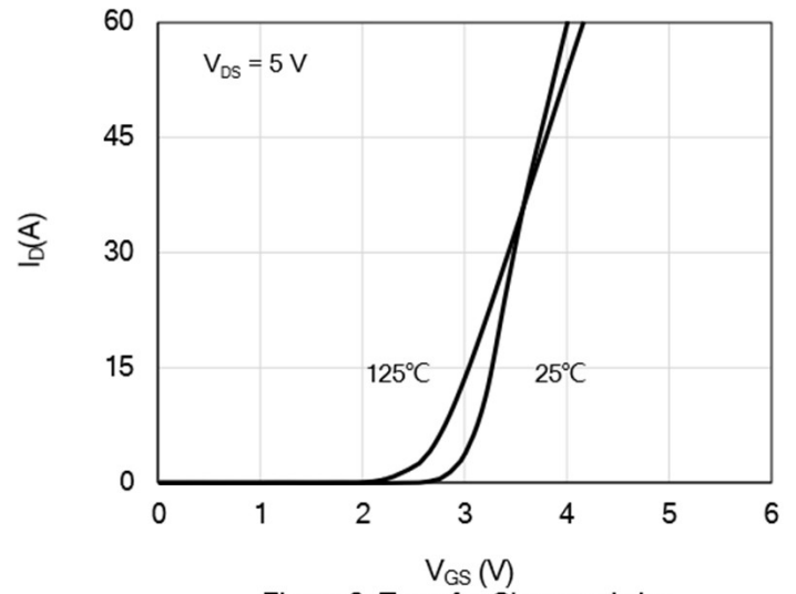
Figure 2: Transfer Characteristics
