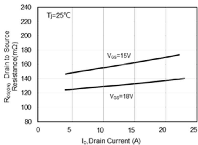
Fig 6. On-Resistance vs Drain Current
