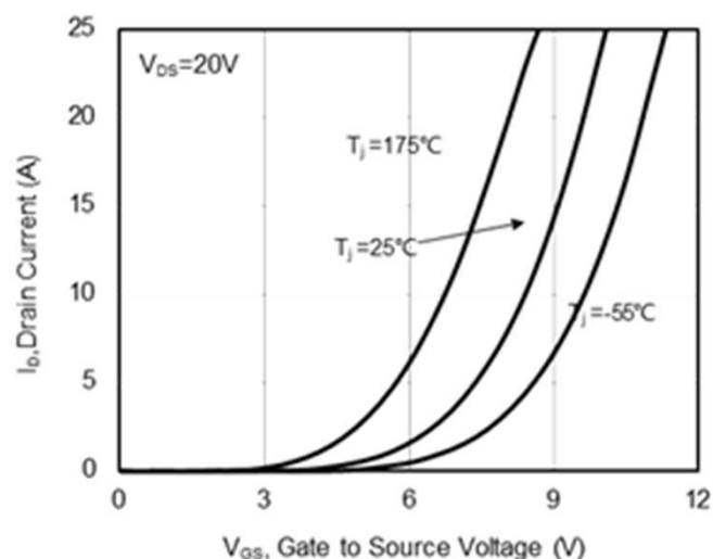
Fig 4. Transfer Characteristics
