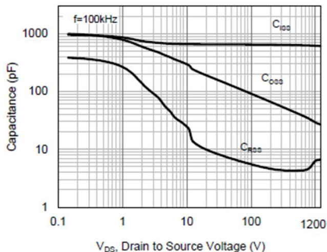
Fig 8. Capacitance Characteristics
