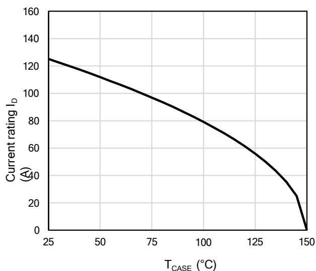
Figure 12: Current De-rating
