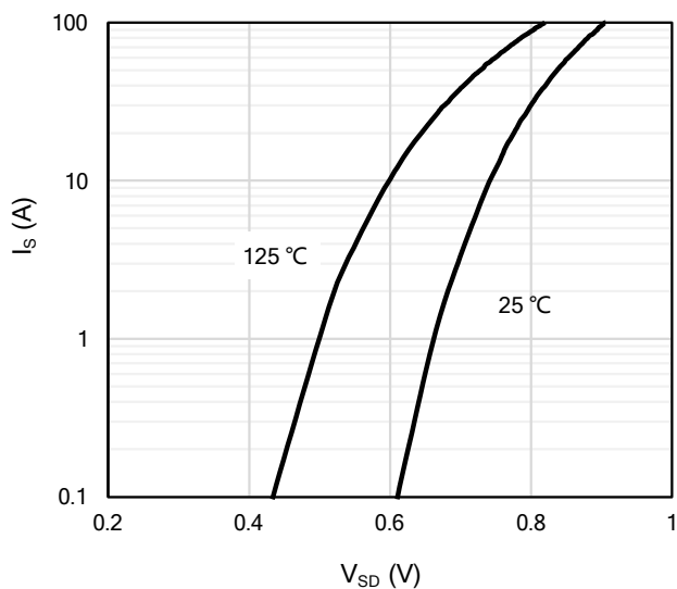
Figure 7: Body-Diode Characteristics
