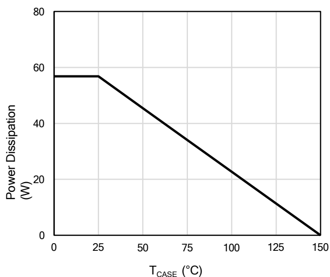
Figure 11: Power De-rating
