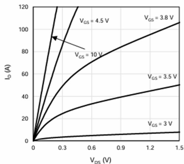
Figure 1: On-Region Characteristics
