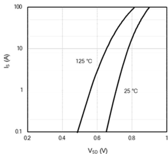
Figure 7: Body-Diode Characteristics
