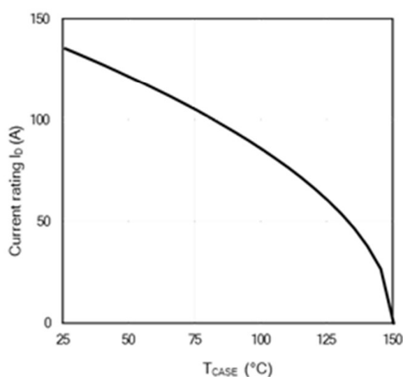
Figure 12: Current De-rating
