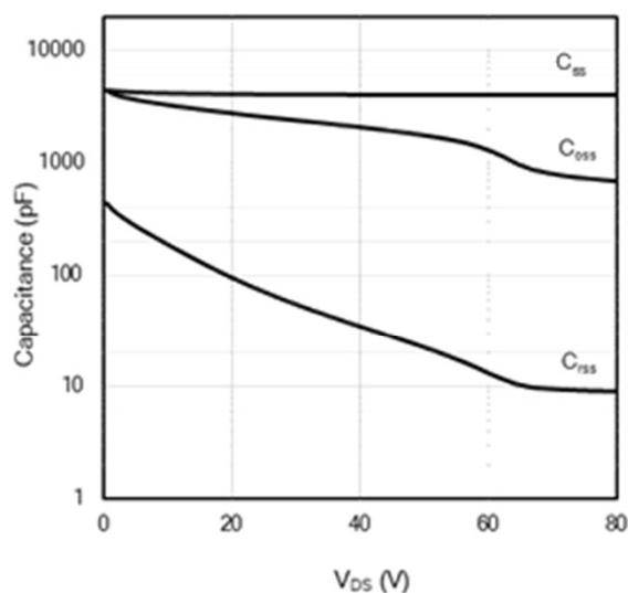
Figure 9: Capacitance Characteristics
