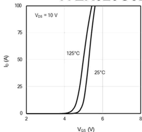
Figure 2: Transfer Characteristics
