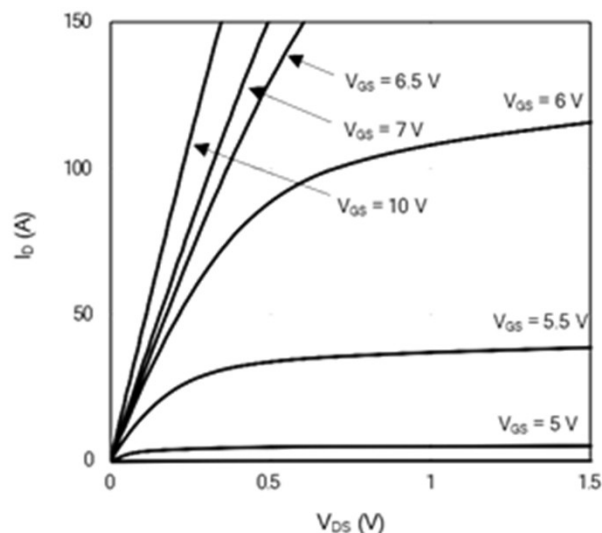
Figure 1: On-Region
