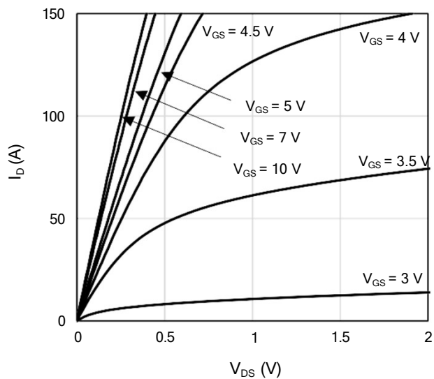
Figure 1: On-Region
