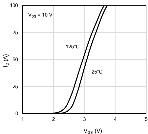
Figure 2: Transfer Characteristics
