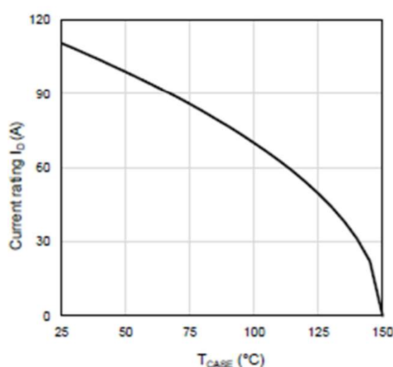
Figure 12: Current De-rating
