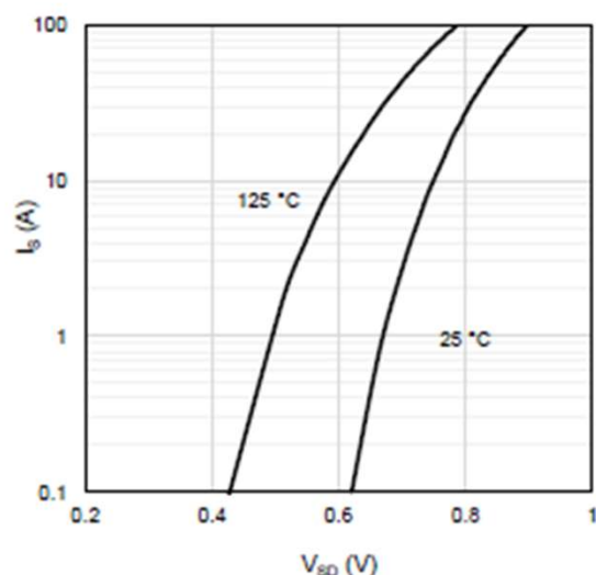
Figure 7: Body-Diode Characteristics
