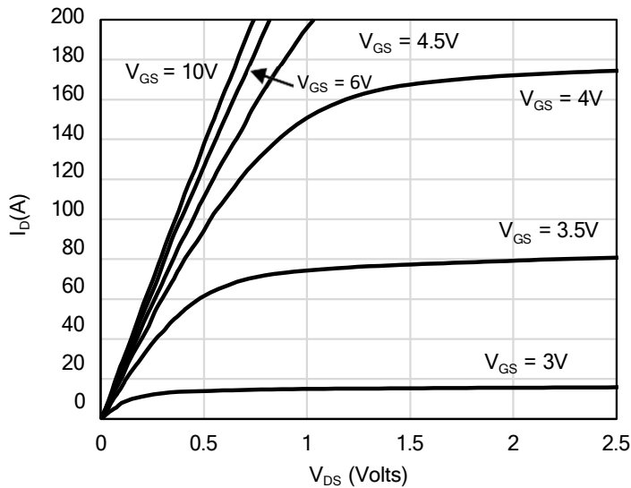
Figure 1: On-Region Characteristics
