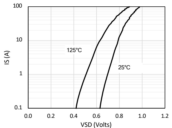
Figure 6: Body-Diode Characteristics
