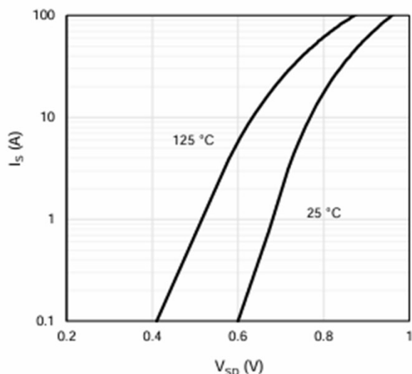
Figure 7: Body-Diode Characteristics
