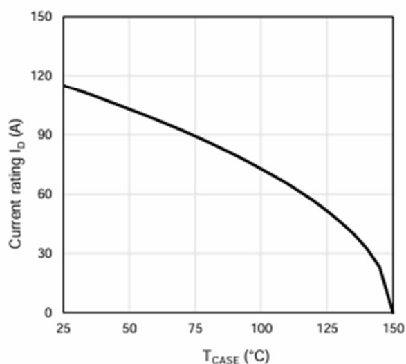
Figure 12: Current De-rating
