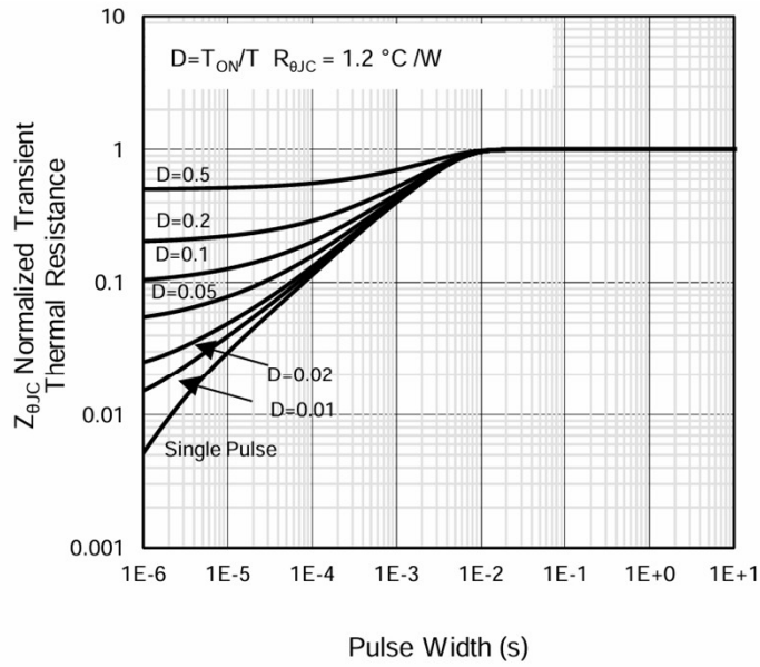
Figure 13: Normalized Maximum Transient Thermal Impedance
