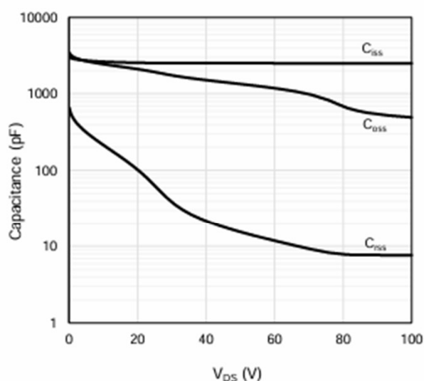
Figure 9: Capacitance Characteristics
