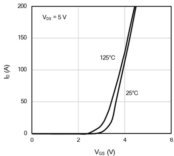
Figure 2: Transfer Characteristics
