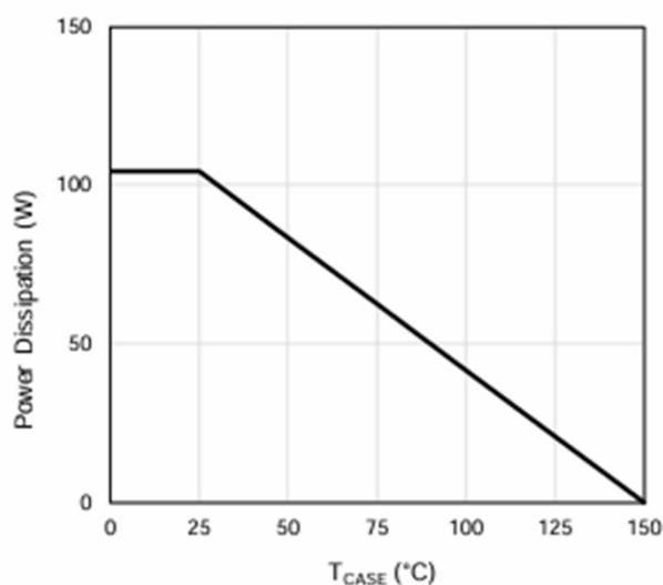
Figure 11: Power De-rating
