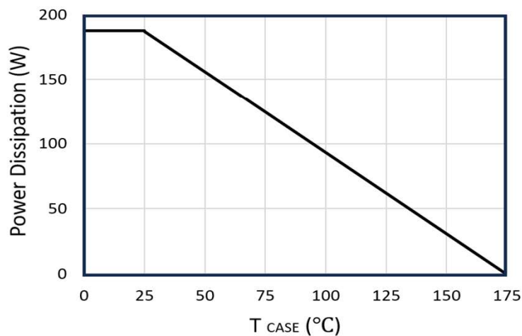
Figure 11: Power De-rating
