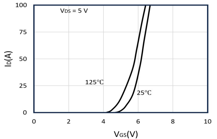
Figure 2: Transfer Characteristic
