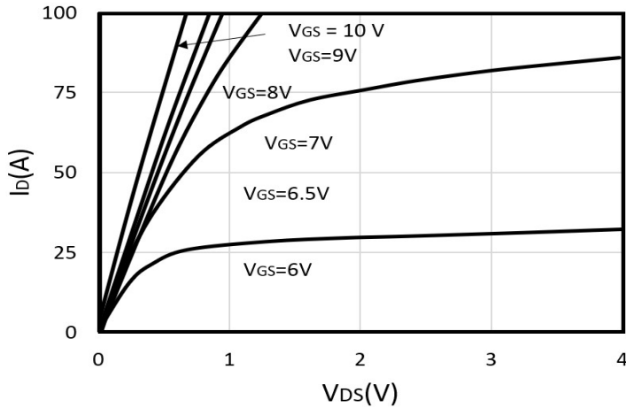
Figure 1: On-Region Characteristics
