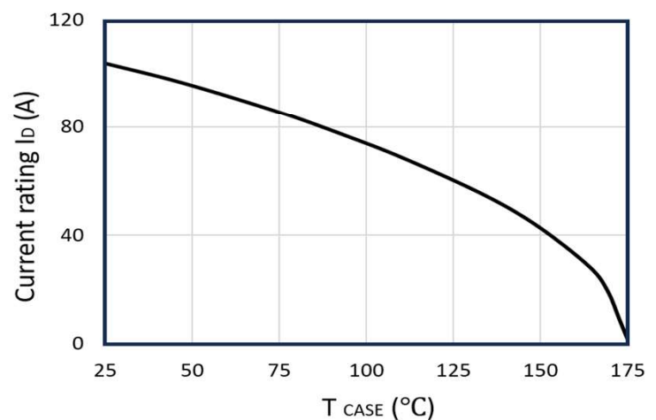
Figure 12: Current De-rating
