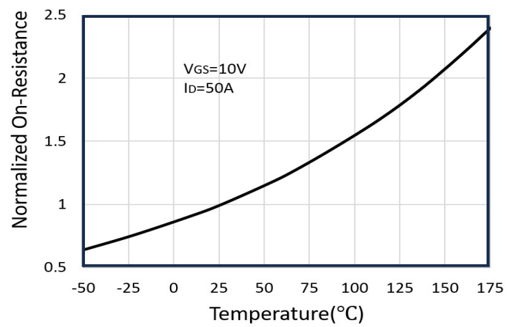
Figure 4: On-Resistance vs. Junction Temperature
