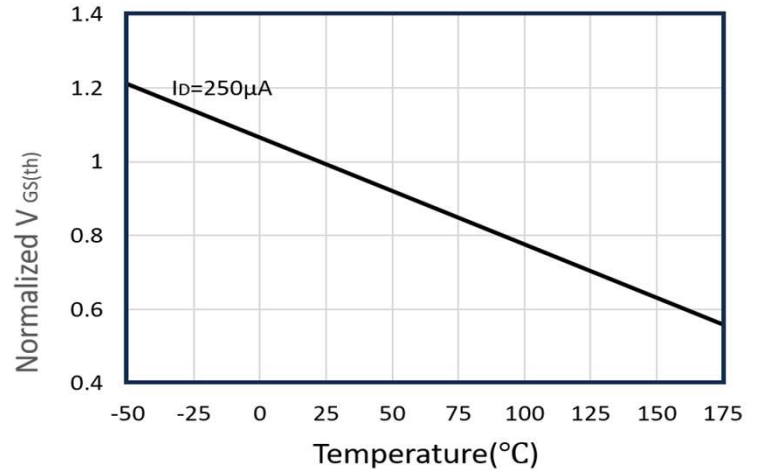
Figure 6: Threshold Voltage vs. Junction Temperature
