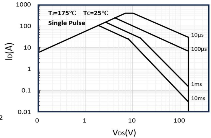
Figure 14: Maximum Forward Biased Safe Operating Area
