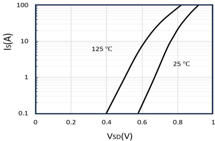
Figure 7: Body-Diode Characteristics
