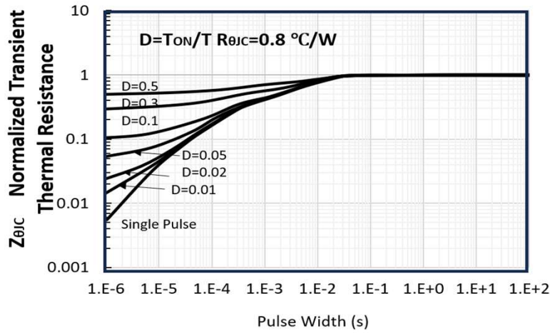
Figure 13: Normalized Maximum Transient Thermal Impedance
