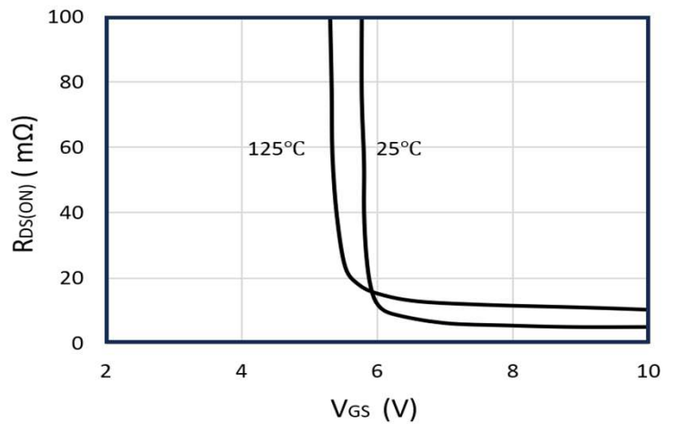
Figure 8: On-Resistance vs. Gate-Source Voltage
