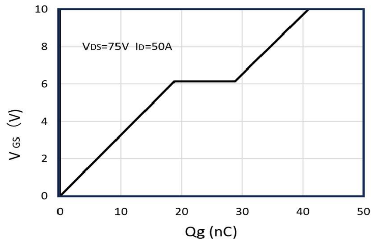
Figure 10: Gate-Charge Characteristics
