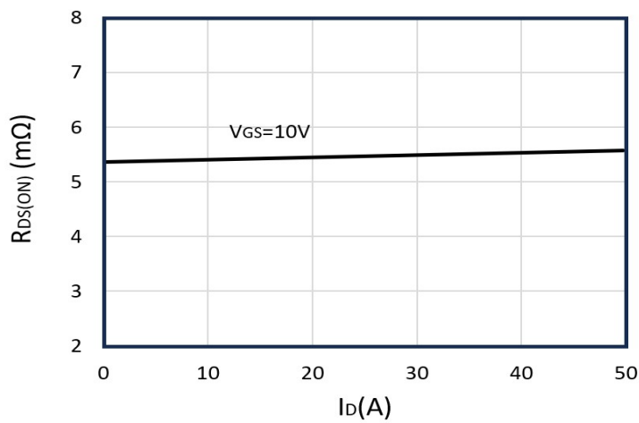
Figure 3: On-Resistance vs. Drain Current and Gate Voltage
