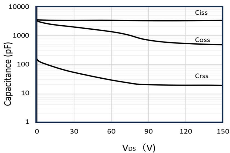
Figure 9: Capacitance Characteristics
