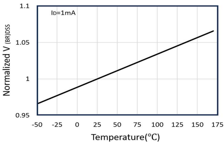
Figure 5: Breakdown Voltage vs. Junction Temperature
