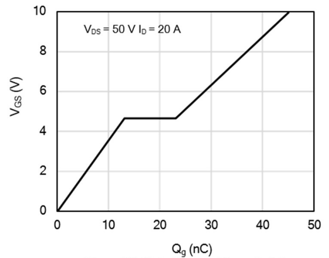
Figure 10: Gate-Charge Characteristics
