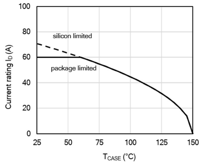
Figure 12: Current De-rating
