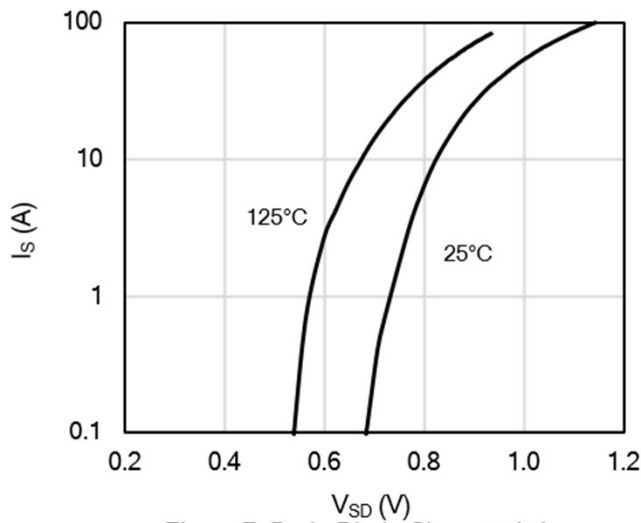
Figure 7: Body-Diode Characteristics
