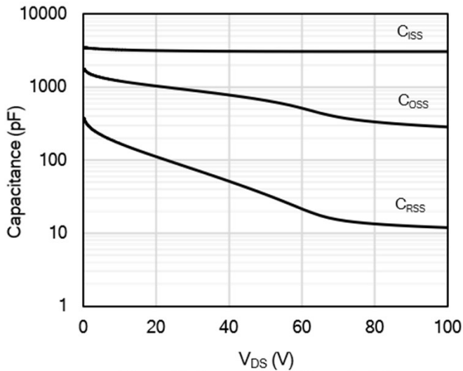
Figure 9: Capacitance Characteristics
