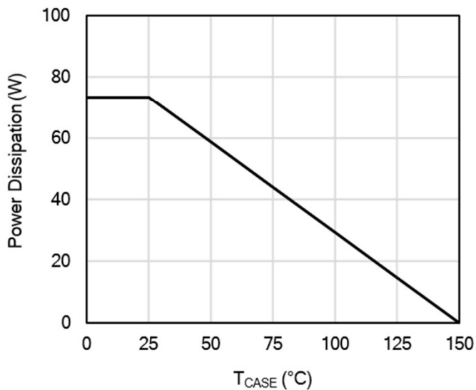
Figure 11: Power De-rating
