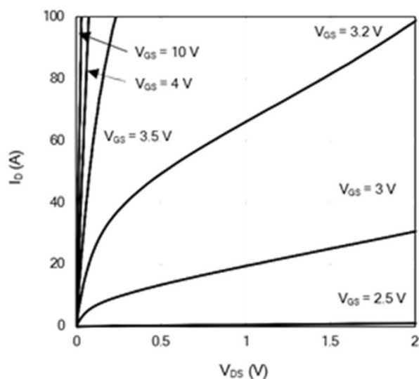
Figure 1: On-Region Characteristics
