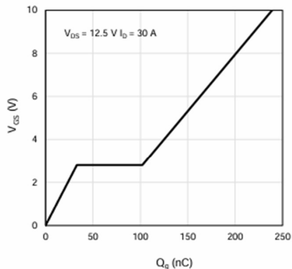
Figure 10: Gate-Charge Characteristics
