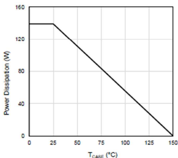
Figure 11: Power De-rating
