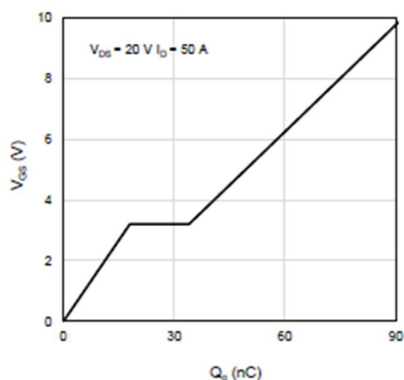
Figure 10: Gate-Charge Characteristics
