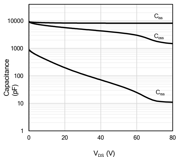
Figure 9: Capacitance Characteristics
