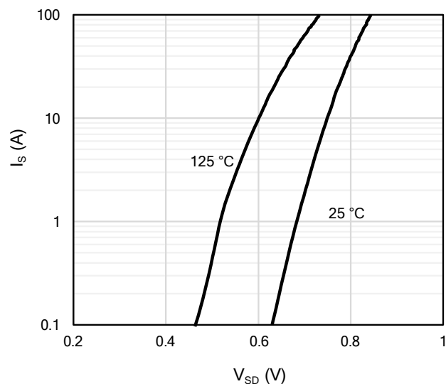
Figure 7: Body-Diode Characteristics
