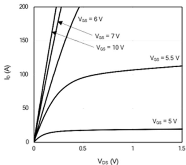
Figure 1: On-Region
