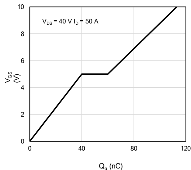
Figure 10: Gate-Charge Characteristics
