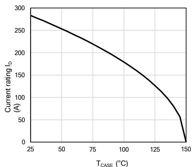
Figure 12: Current De-rating
