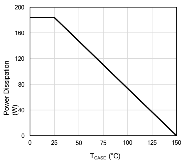
Figure 11: Power De-rating
