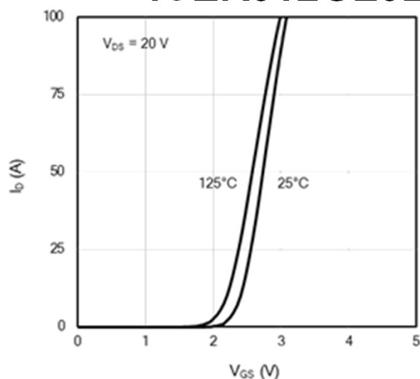
Figure 2: Transfer Characteristics
