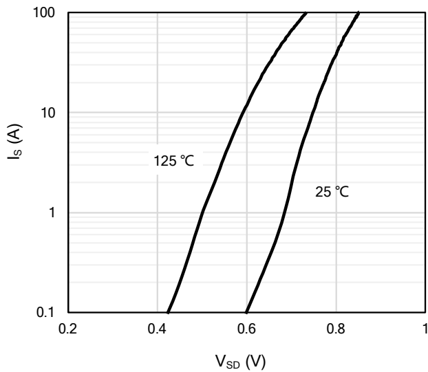
Figure 7: Body-Diode Characteristics
