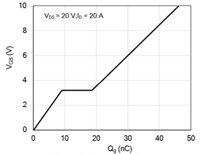
Figure 10: Gate-Charge Characteristics
