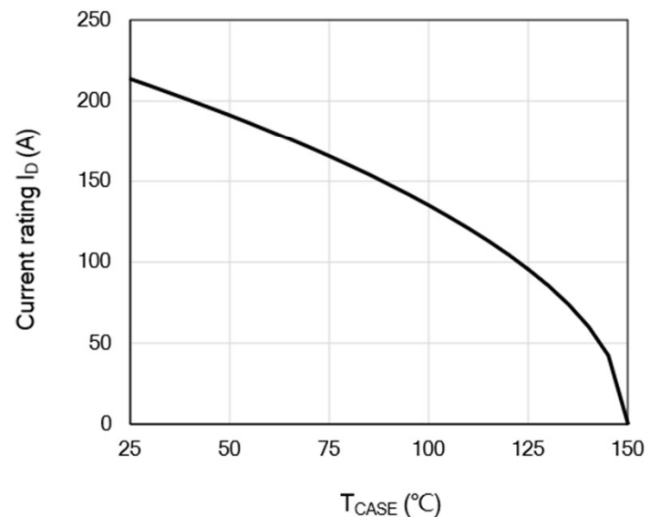
Figure 12: Current De-rating
