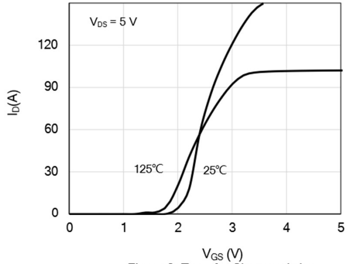
Figure 2: Transfer Characteristics
