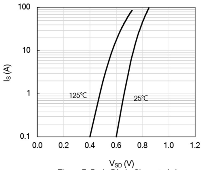
Figure 7: Body-Diode Characteristics
