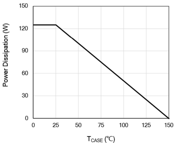
Figure 11: Power De-rating
