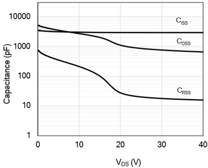
Figure 9: Capacitance Characteristics
