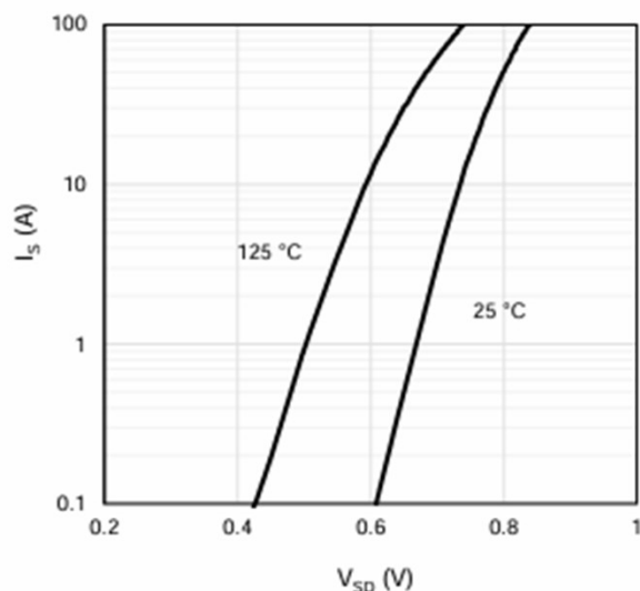
Figure 7: Body-Diode Characteristics
