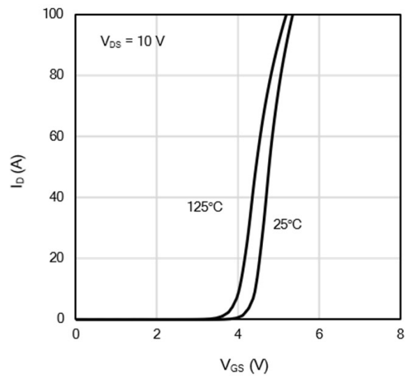
Figure 2: Transfer Characteristics
