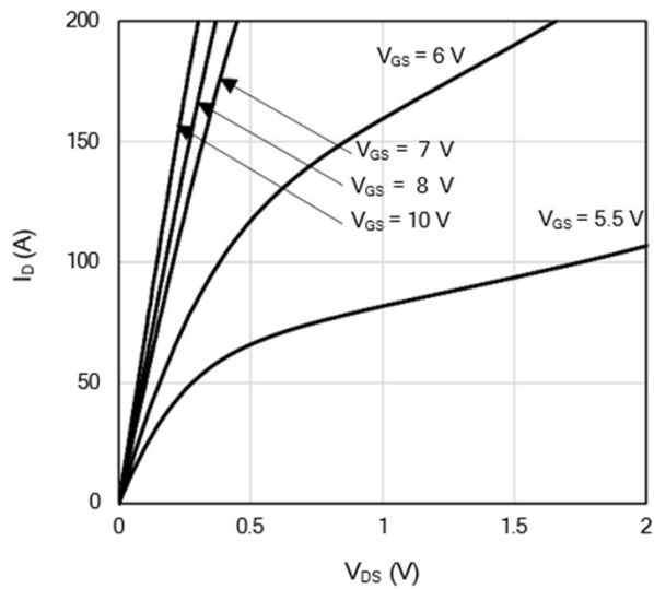
Figure 1: On-Region
