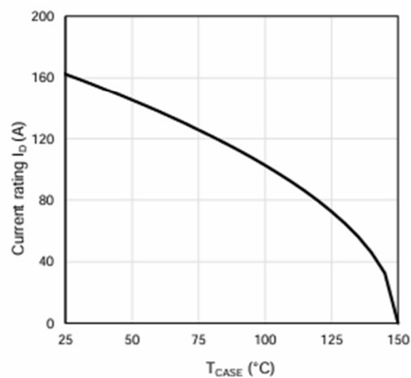
Figure 12: Current De-rating
