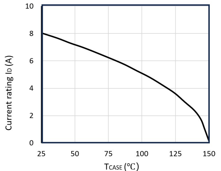
Figure 12: Current De-rating
