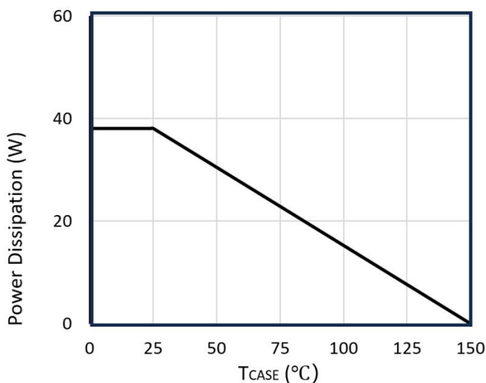
Figure 11: Power De-rating
