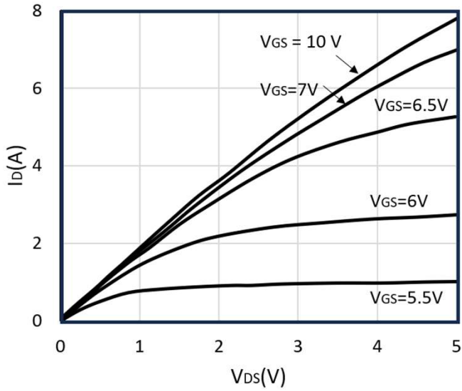
Figure 1: On-Region Characteristics
