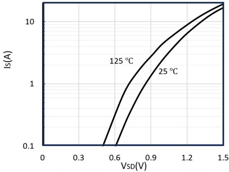
Figure 7: Body-Diode Characteristics
