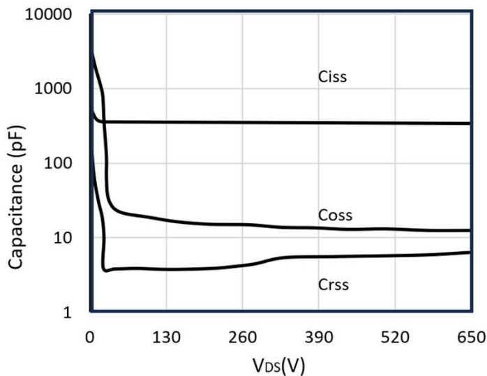
Figure 9: Capacitance Characteristics
