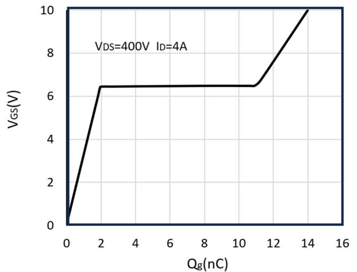
Figure 10: Gate-Charge Characteristics
