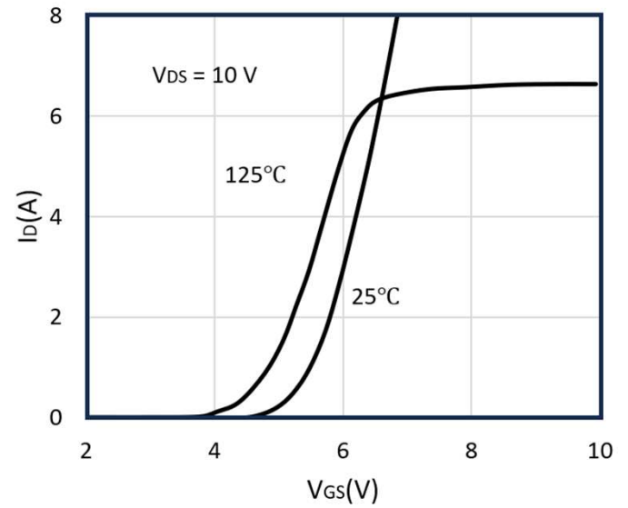
Figure 2: Transfer Characteristic
