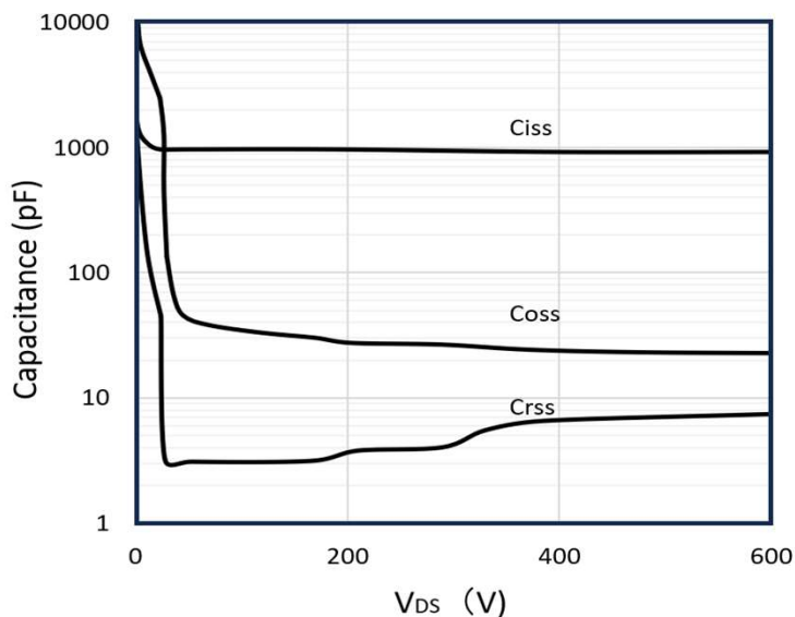
Figure 9: Capacitance Characteristics
