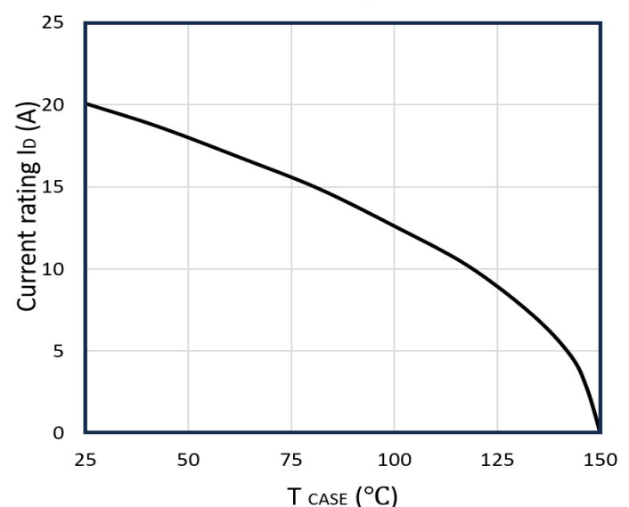
Figure 12: Current De-rating
