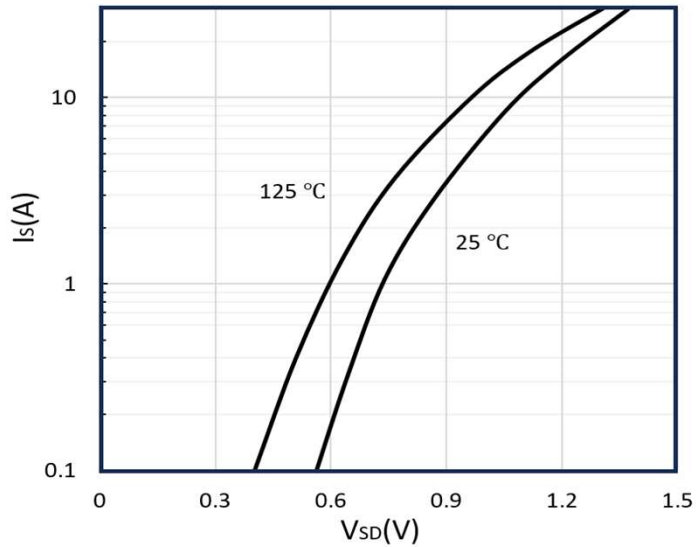
Figure 7: Body-Diode Characteristics
