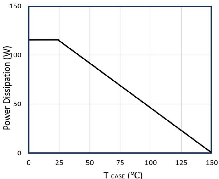
Figure 11: Power De-rating
