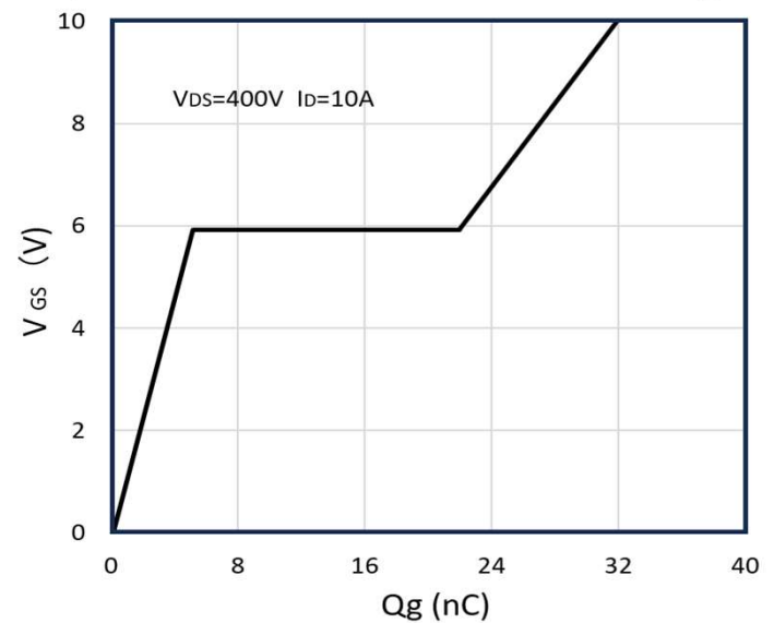
Figure 10: Gate-Charge Characteristics
