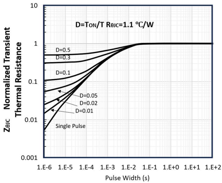
Figure 13: Normalized Maximum Transient Thermal Impedance
