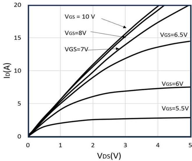
Figure 1: On-Region Characteristics
