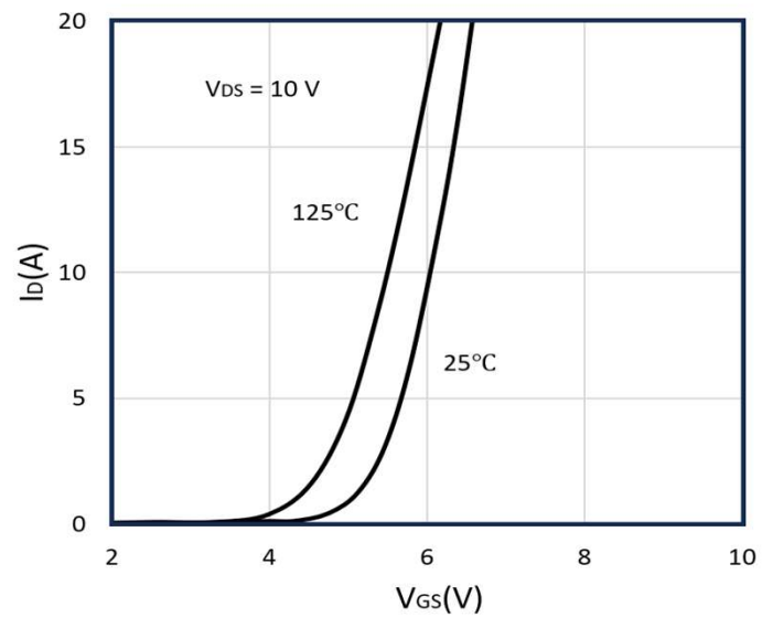
Figure 2: Transfer Characteristic
