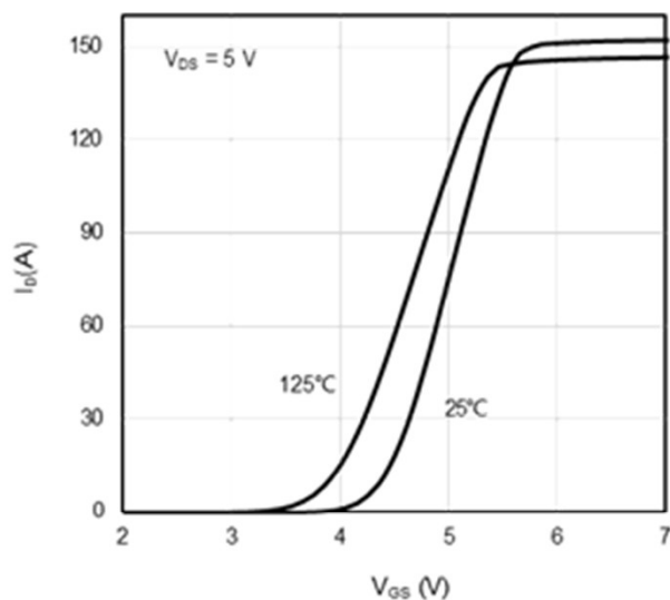
Figure 2: Transfer Characteristics
