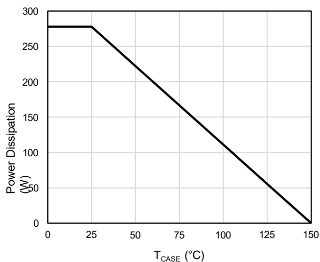
Figure 11: Power De-rating
