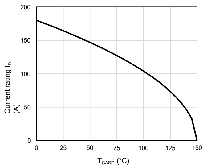
Figure 12: Current De-rating
