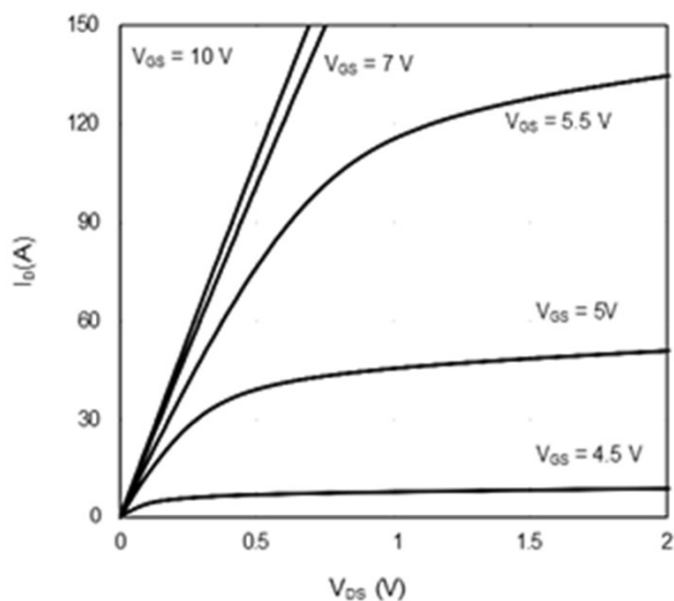
Figure 1: On-Region Characteristics
