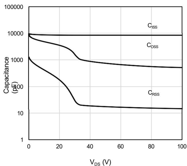
Figure 9: Capacitance Characteristics
