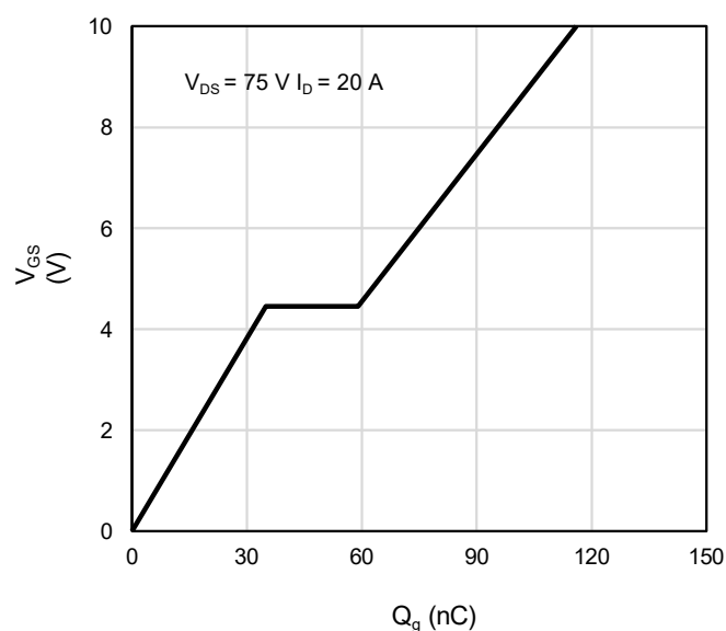
Figure 10: Gate-Charge Characteristics
