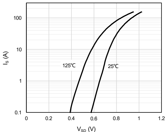
Figure 7: Body-Diode Characteristics
