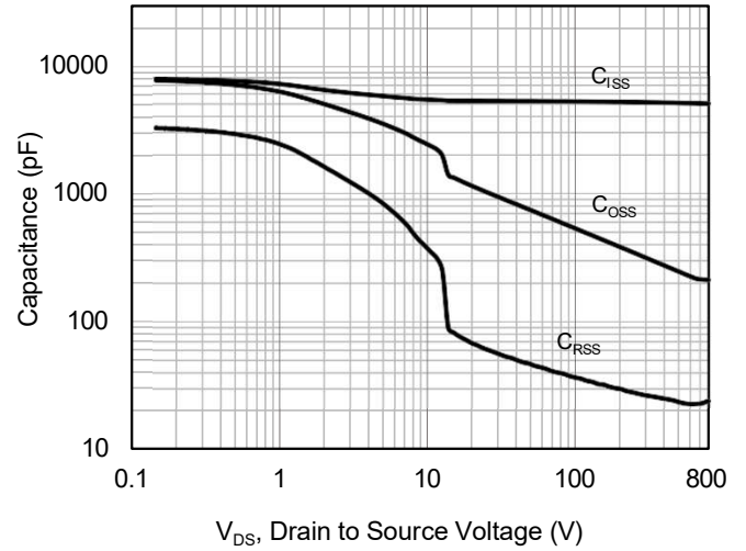
Fig 8. Capacitance Characteristics
