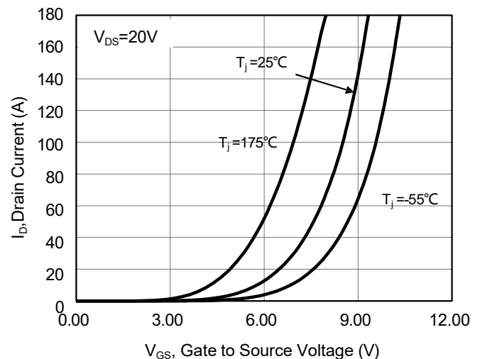
Fig 4. Transfer Characteristics
