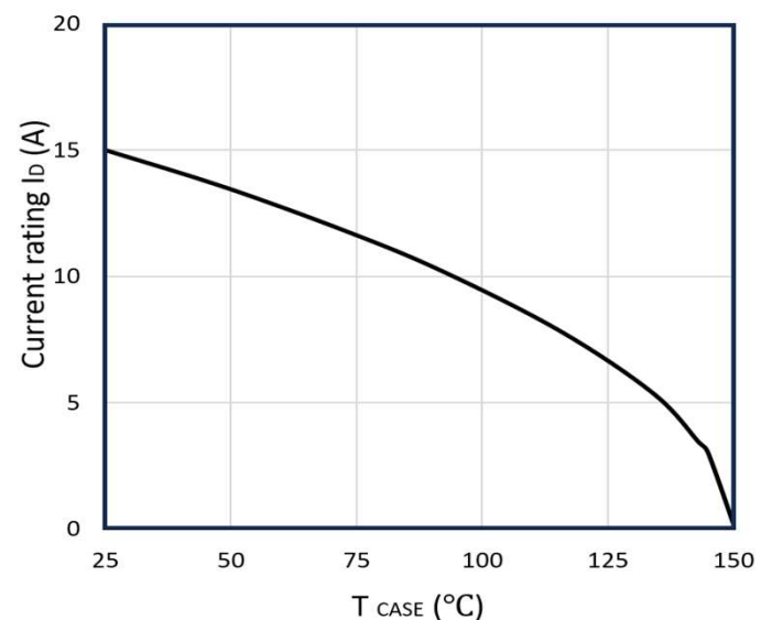
Figure 12: Current De-rating
