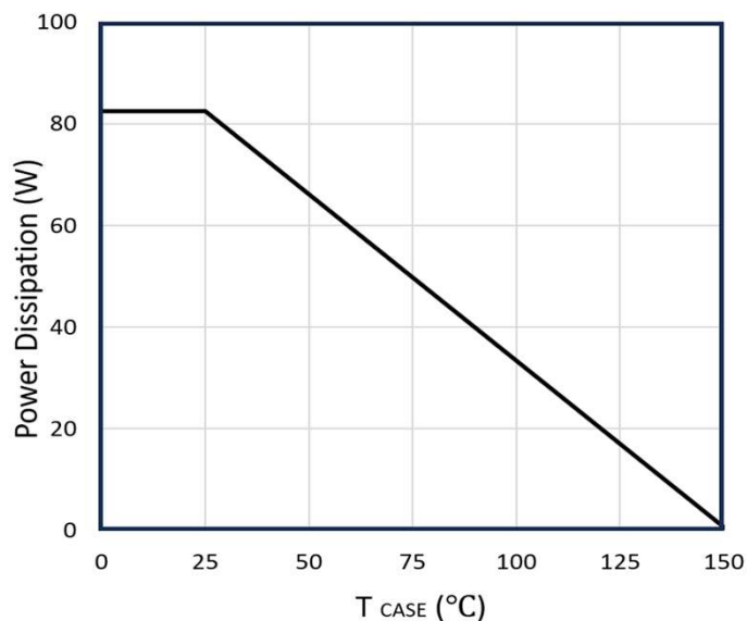
Figure 11: Power De-rating
