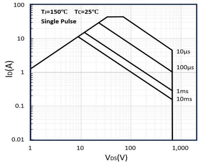
Figure 14: Maximum Forward Biased Safe Operating Area
