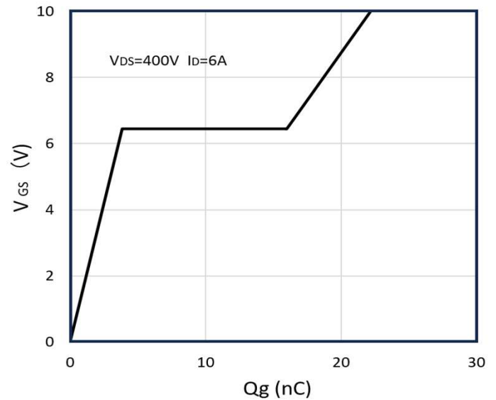
Figure 10: Gate-Charge Characteristics
