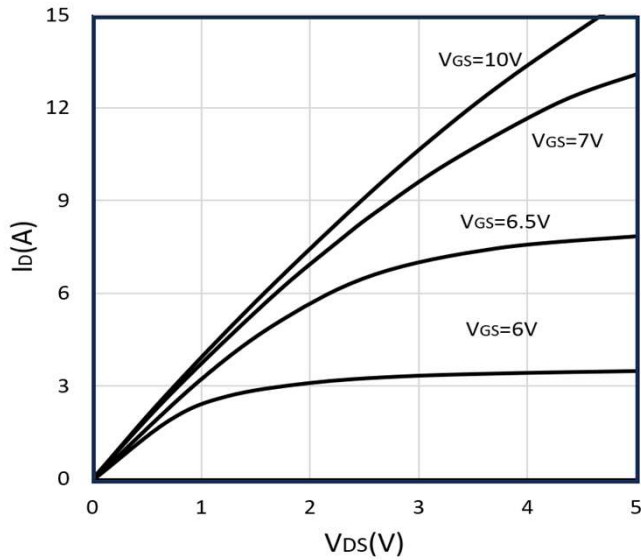
Figure 1: On-Region Characteristics
