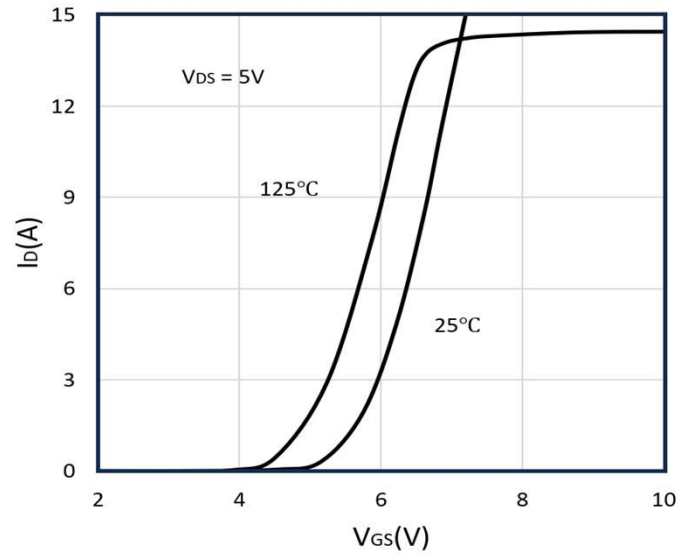
Figure 2: Transfer Characteristic
