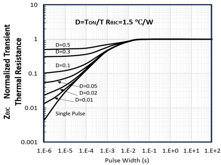
Figure 13: Normalized Maximum Transient Thermal Impedance
