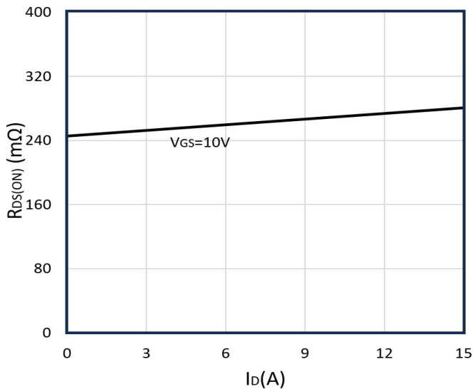
Figure 3: On- Resistance vs. Drain Current and Gate Voltage
