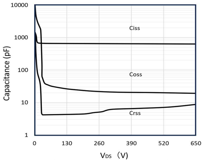
Figure 9: Capacitance Characteristics
