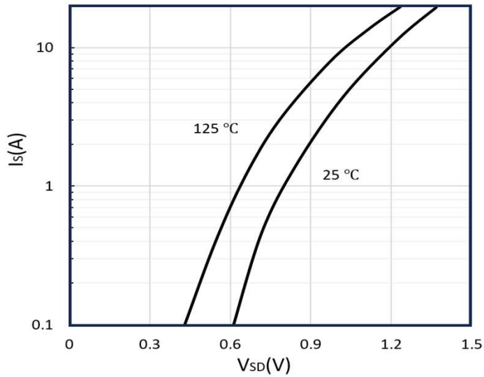
Figure 7: Body-Diode Characteristics
