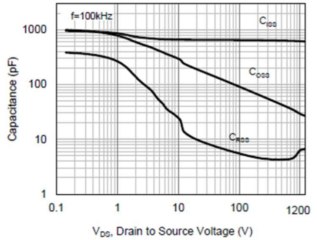
Fig 8. Capacitance Characteristics
