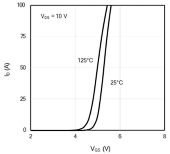
Figure 2: Transfer Characteristics
