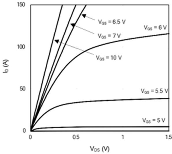
Figure 1: On-Region
