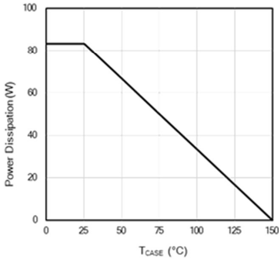
Figure 11: Power De-rating
