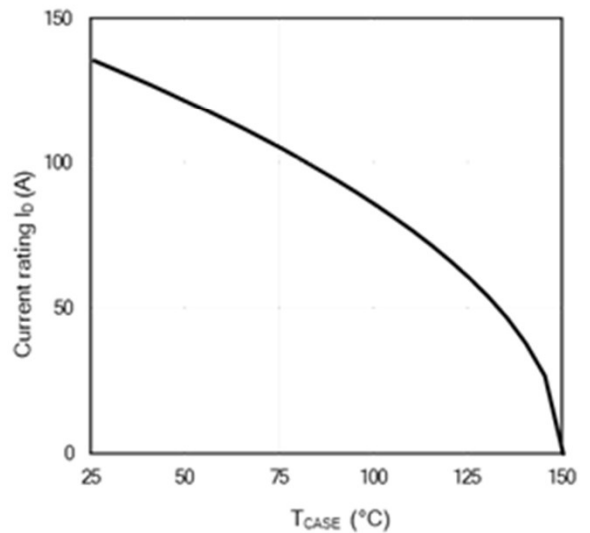
Figure 12: Current De-rating
