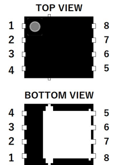
DFN5x6
