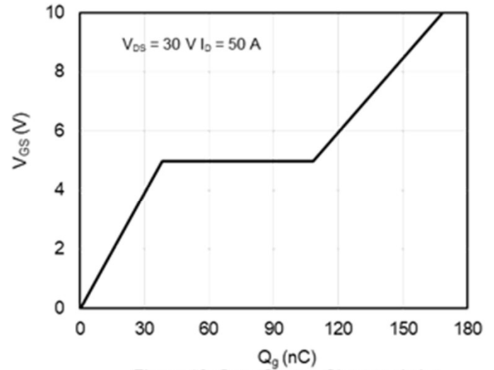
Figure 10: Gate-Charge Characteristics
