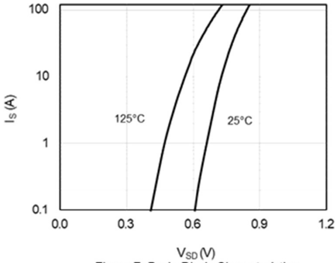
Figure 7: Body-Diode Characteristics
