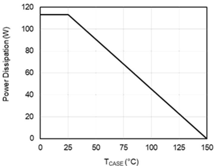
Figure 11: Power De-rating
