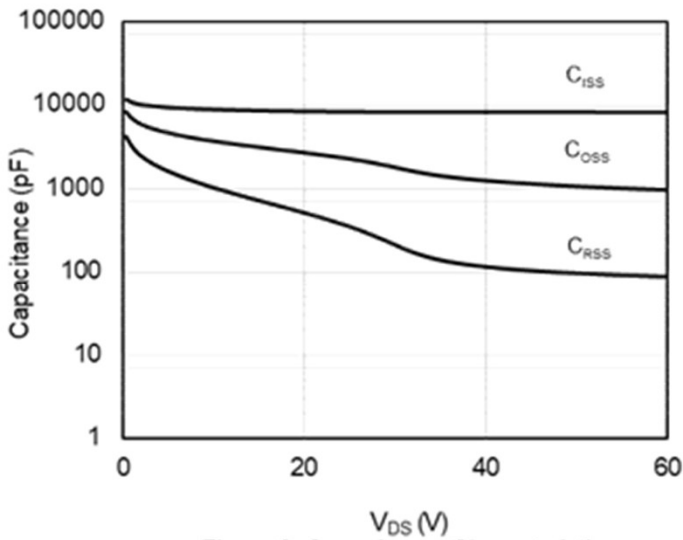
Figure 9: Capacitance Characteristics
