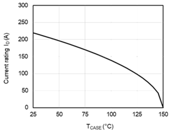
Figure 12: Current De-rating
