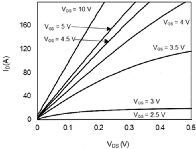
Figure 1: On-Region Characteristics
