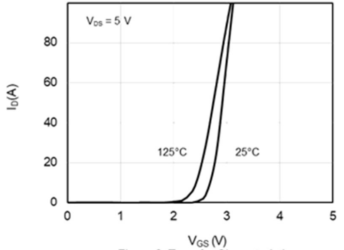
Figure 2: Transfer Characteristics
