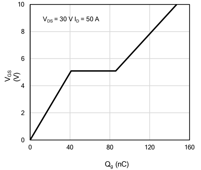
Figure 10: Gate-Charge Characteristics
