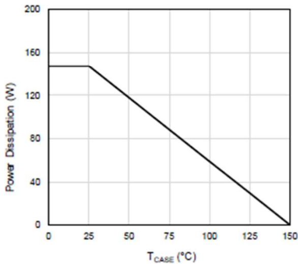
Figure 11: Power De-rating
