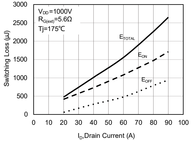
Fig 10. Switching Energy vs. Drain Current
