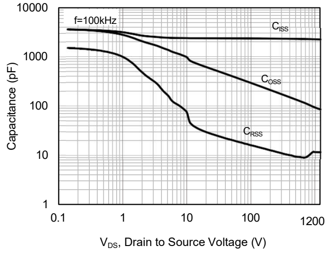
Fig 8. Capacitance Characteristics
