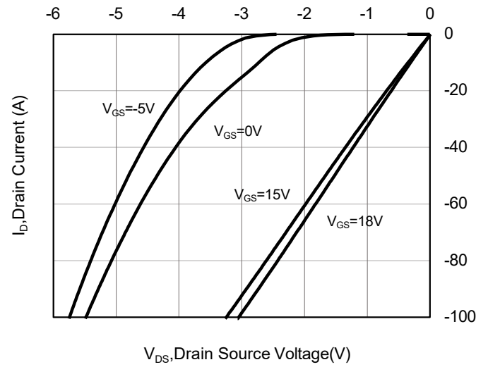
Fig 14. 3rd Quadrant Characteristic at 25 °C
