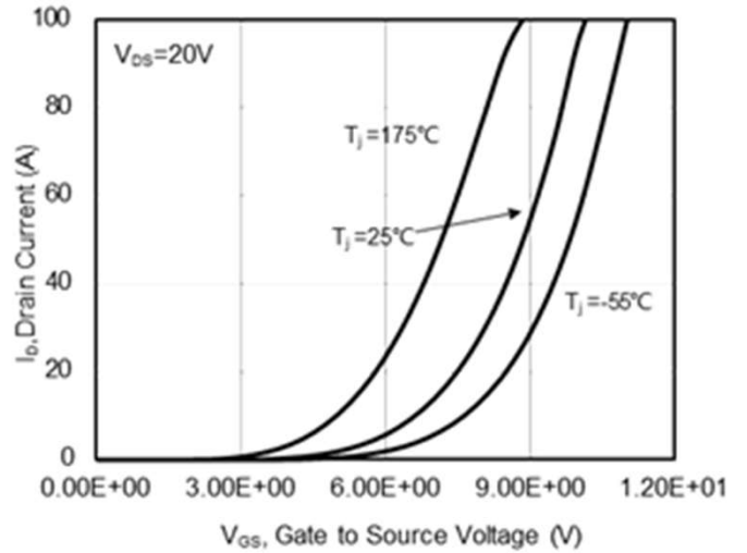
Fig 4. Transfer Characteristics
