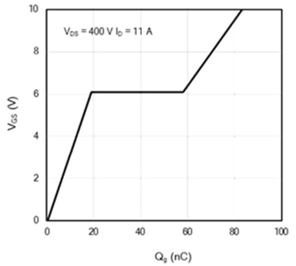
Figure 10: Gate-Charge Characteristics
