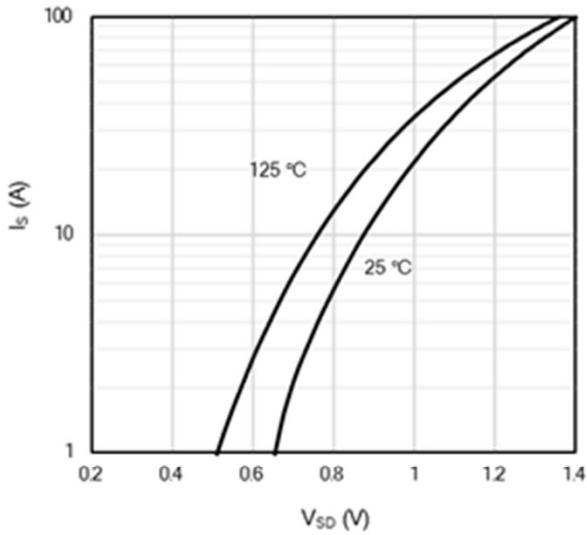
Figure 7: Body-Diode Characteristics
