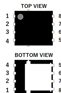
DFN5x6
