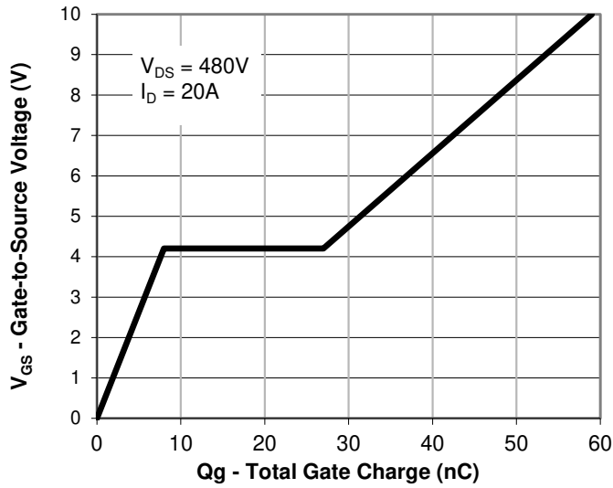
Gate Charge
