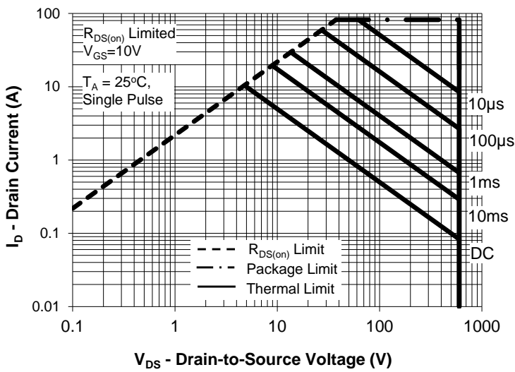
Full Pak TO-220 Package Maximum Rated Forward Biased SOA
