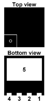
DFN8x8
