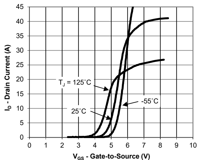
Transfer Characteristics
